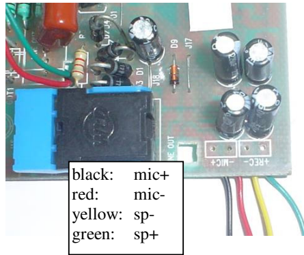
Figure 2.1 Handset wire connection to the board.
