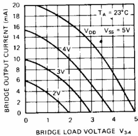
BRIDGE OUTPUT CURRENT VS. BRIDGE OUTPUT VOLTAGE
