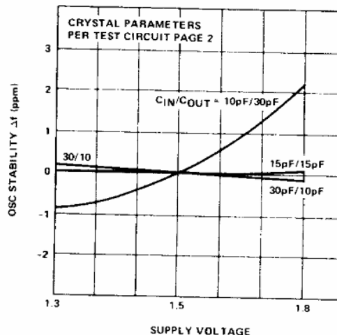
OSCILLATOR STABILITY VS. SUPPLY VOLTAGE
