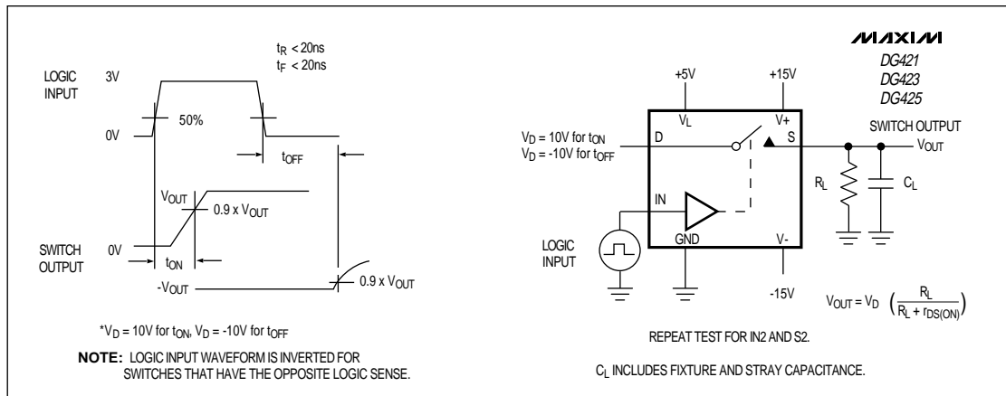
Figure 2. Switching Time
