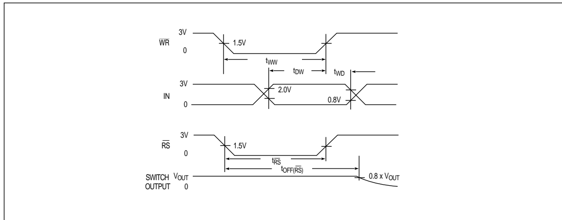
Figure 3. Latch Timing
