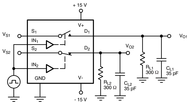
Figure 2. Break-Before-Make (DG456)
