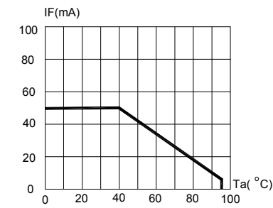
FIG.5 RED & AMBER MAXIMUM FORWARD DC CURRENT VS AMBIENT TEMPERATURE ( T_{jmax}=105^{\circ}C )
