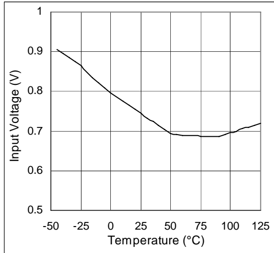
Figure 9. Minimum Input Startup Voltage vs. Temp.
