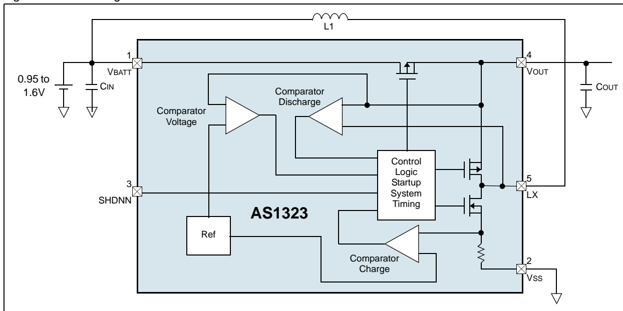
Figure 11. Block Diagram
