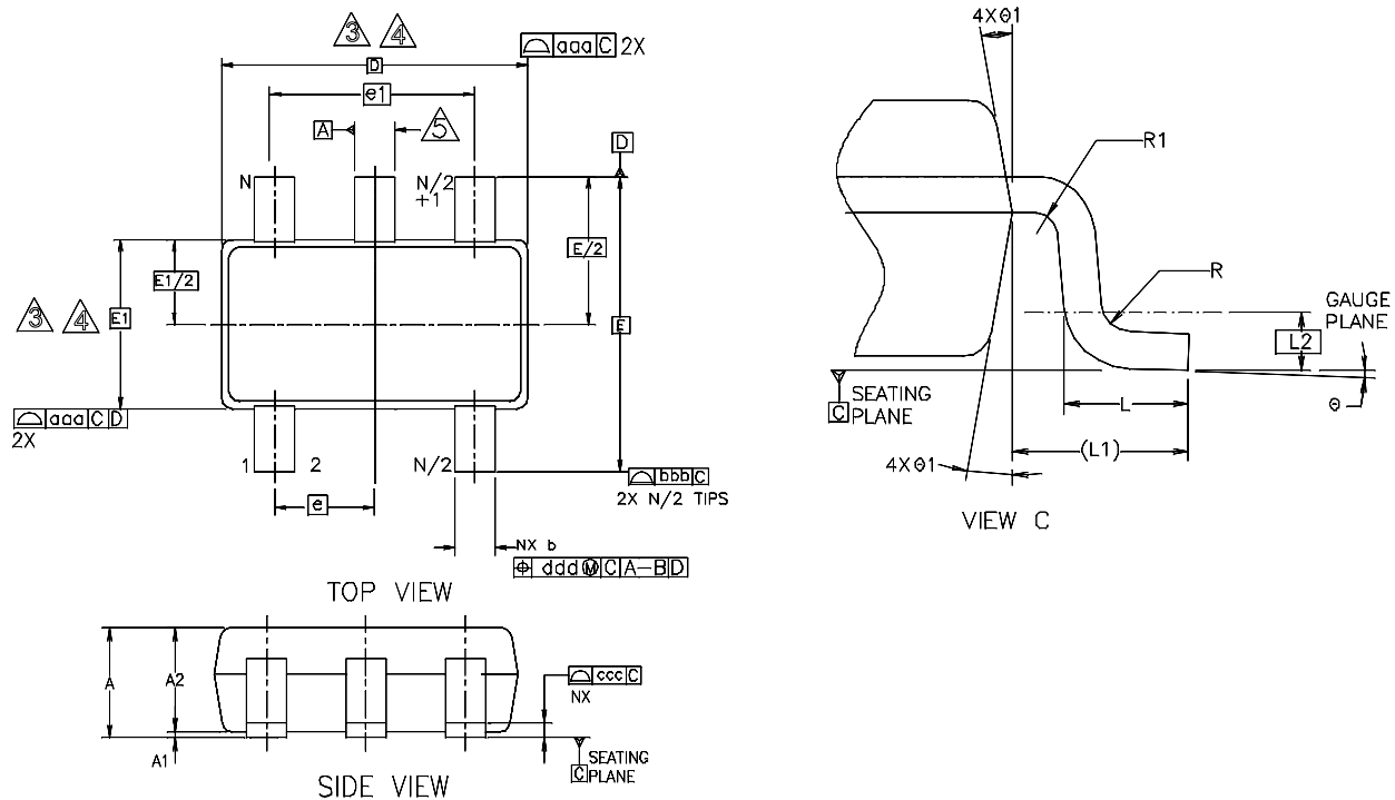
Figure 13. TSOT23-5 Package
