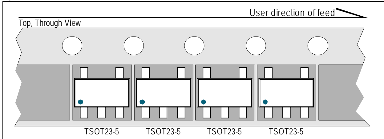
Figure 14. Tape&Reel Pin1 Orientation
