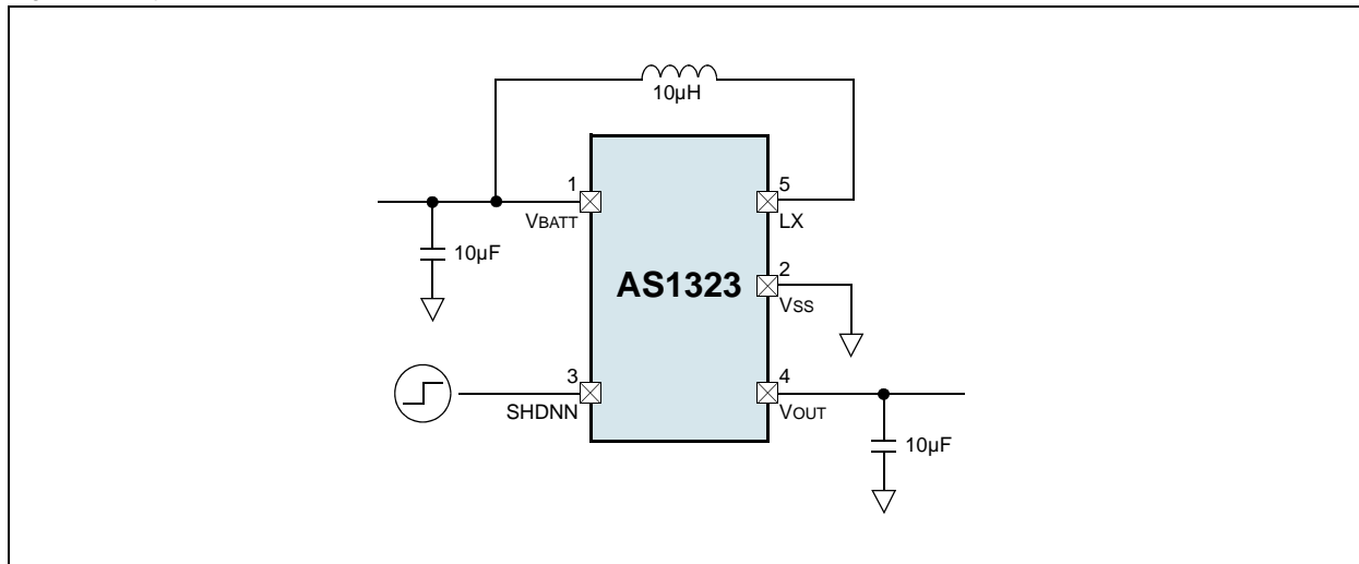
Figure 12. Typical Application
