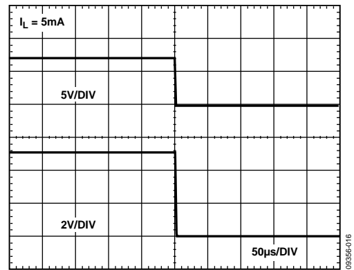
Figure 12. Turn-Off Time
