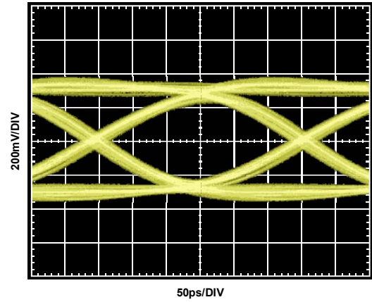
Figure 22. 3.25 Gbps Output Eye, 40 Inch FR4 Output Channel, PE = Best Setting (TP3 from Figure 19)
