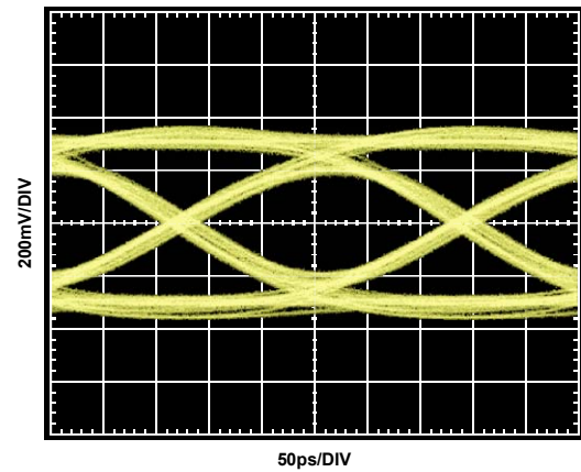
Figure 23. 3.75 Gbps Output Eye, 40 Inch FR4 Output Channel, PE = Best Setting (TP3 from Figure 19)
