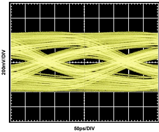
Figure 21. 3.75 Gbps Output Eye, 40 Inch FR4 Output Channel, PE = 0 (TP3 from Figure 19)
