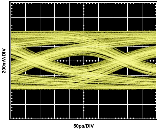
Figure 20. 3.25 Gbps Output Eye, 40 Inch FR4 Output Channel, PE = 0 (TP3 from Figure 19)
