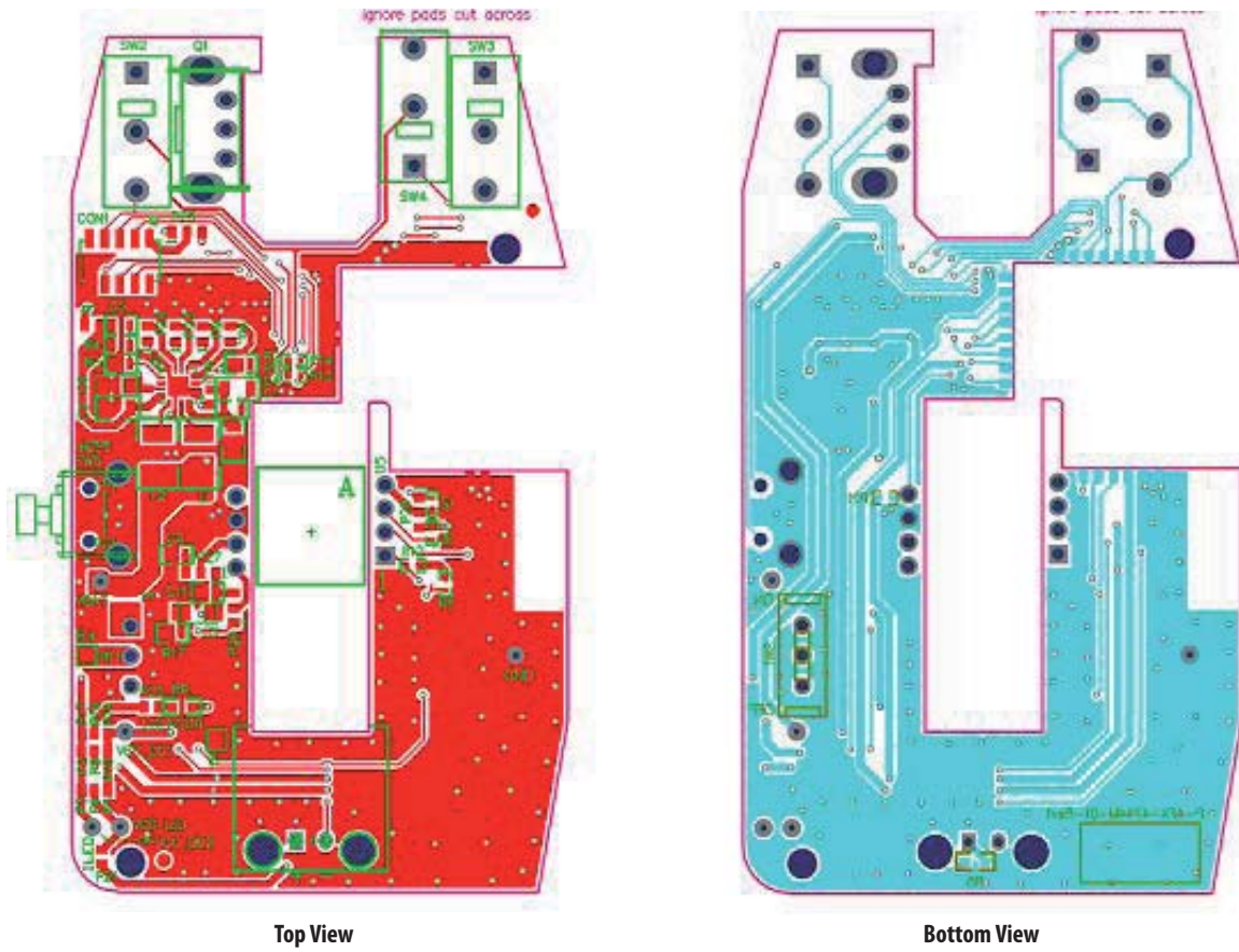
Figure C1. PCB layout for main board of ADNK-3003-ND24 wireless Optical mouse designer's kit
