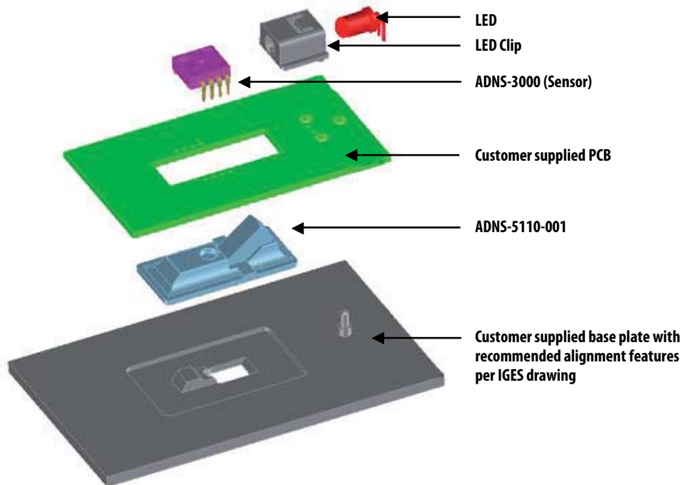
Figure 4. Exploded view drawing of optical tracking engine with ADNS-3000 Optical mouse sensor
