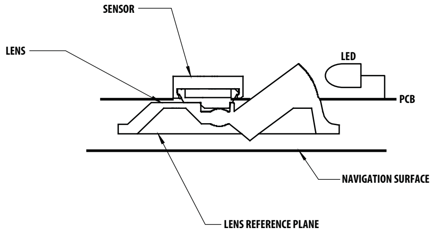
Figure E1. Optical System Assembly Cross Sectional View
