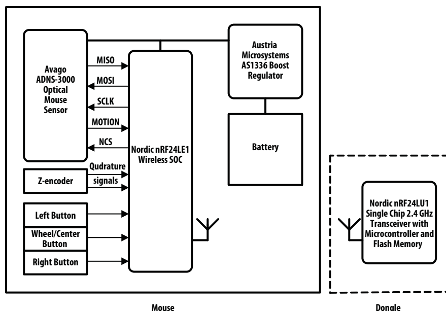
Figure 1. ADNK-3003-ND24 Reference Design Mouse Functional Block Diagram
