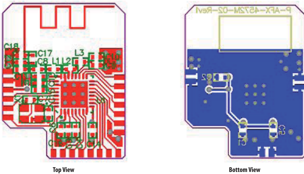
Figure C2. PCB layout ADNK-3003-ND24 Designer's Kit RF module
