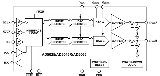
Figure 1. AD5025/45/65
