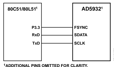
Figure 36. 80C51/80L51 to AD5932 Interface
