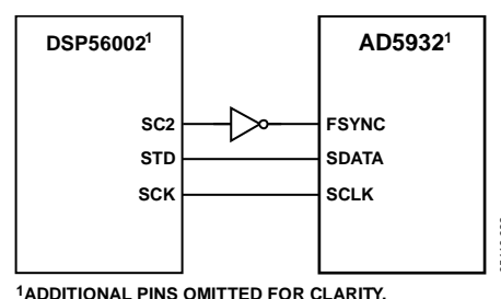
Figure 37. DSP56002 to AD5932 Interface
