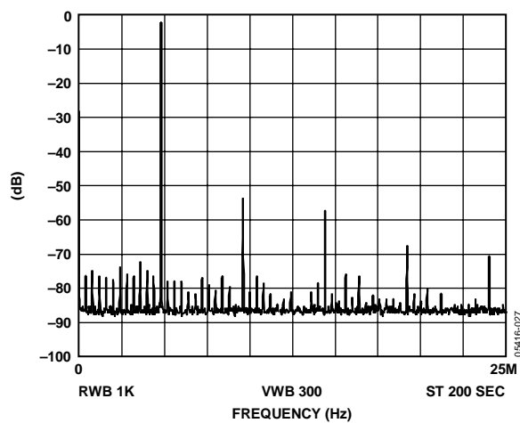
Figure 27. f_{MCLK} = 50 MHz, f_{OUT} = 4.8 MHz, Frequency Word = 189374C
