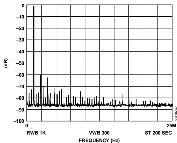
Figure 26. f_{MCLK} = 50 MHz, f_{OUT} = 1.2 MHz, Frequency Word = 0624DD3
