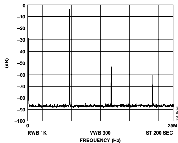
Figure 28. f_{MCLK} = 50 MHz, f_{OUT} = 7.143 MHz = f_{MCLK}/7 , Frequency Word = 2492492
