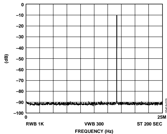
Figure 29. f_{MCLK} = 50 MHz, f_{OUT} = 16.667 MHz = f_{MCLK}/3 , Frequency Word = 5555555
