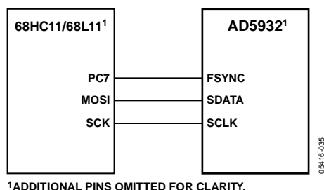
Figure 35. 68HC11/68L11 to AD5932 Interface
