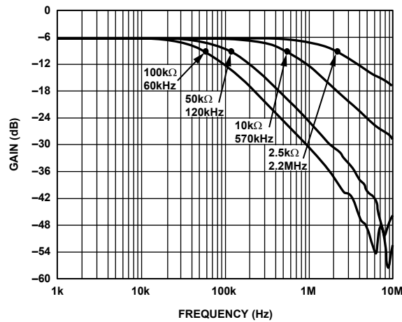
Figure 22. -3\text{ dB} Bandwidth @ Code = 0x80
