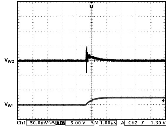
Figure 26. Analog Crosstalk
