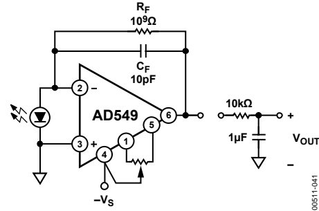
Figure 41. Photodiode Preamp
