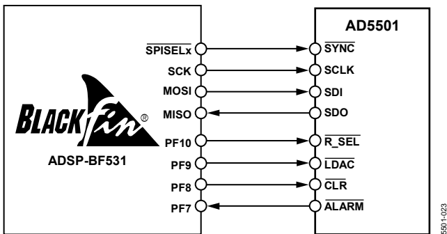
Figure 13. Interfacing to a Blackfin DSP
