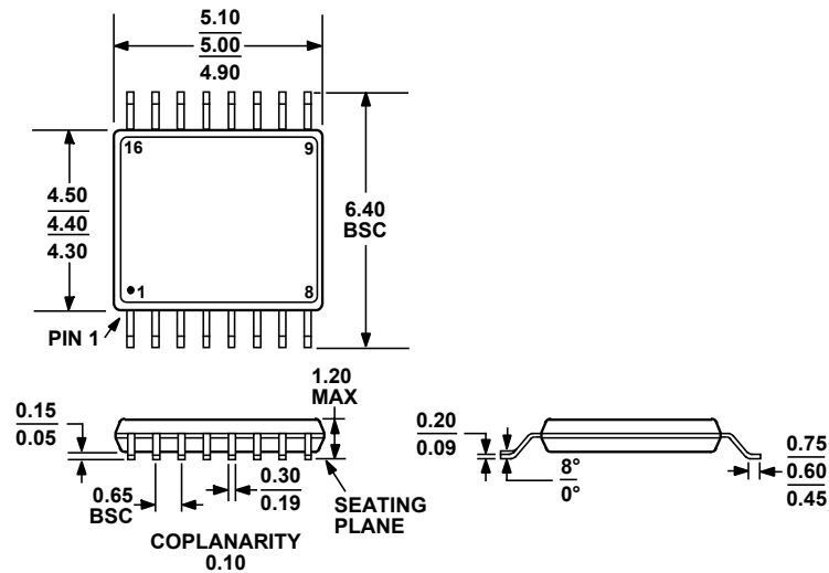
Figure 15. 16-Lead Thin Shrink Small Outline Package [TSSOP] (RU-16) Dimensions shown in millimeters
