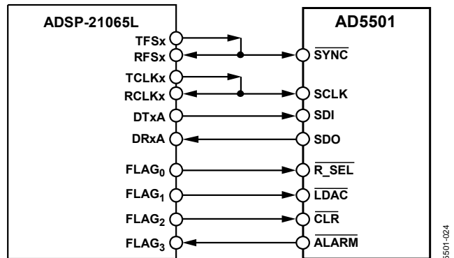
Figure 14. Interfacing to an ADSP-21065L DSP
