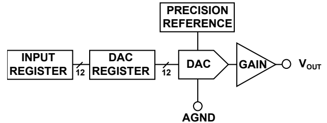
Figure 11. DAC Channel Architecture
