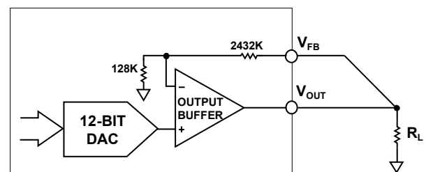
Figure 12. V_{FB} and V_{OUT} force-sense configuration
