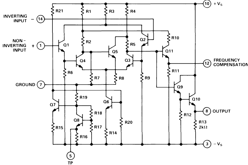
Figure 12. AD5539 Circuit
