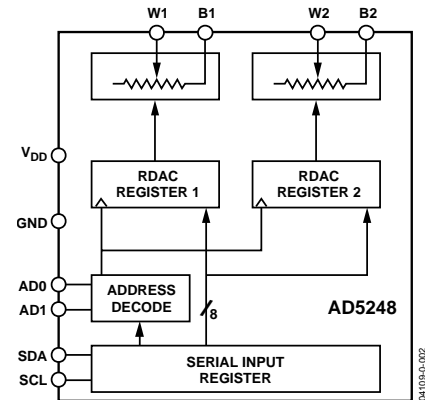
Figure 2. AD5248
