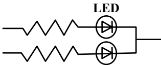
(A) Recommended circuit
