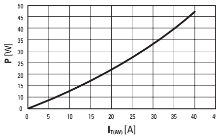
Fig. 1: Power dissipation versus average on-state current.
