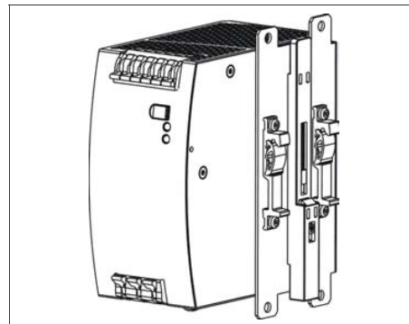
Fig. 24-4 Side Mounting with DIN-rail brackets
