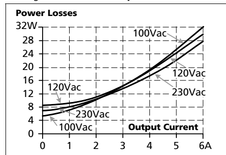
Fig. 9-2 Losses vs. output current at 48V
