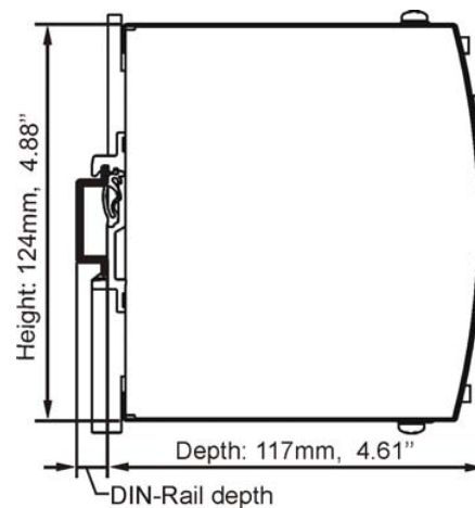
Fig. 22-2 Side view
