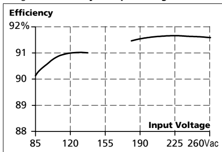
Fig. 9-3 Efficiency vs. input voltage, 48V, 5A
