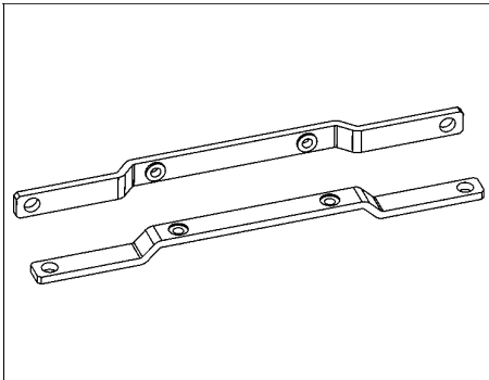
Fig. 24-1 ZM1.WALL Wall Mounting Bracket
