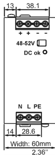
Fig. 22-1 Front view
