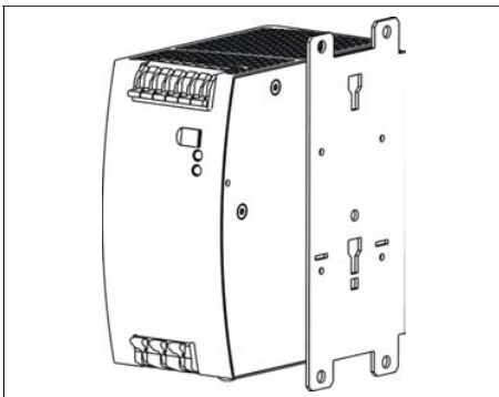
Fig. 24-3 ZM13.SIDE Side Mounting Bracket
