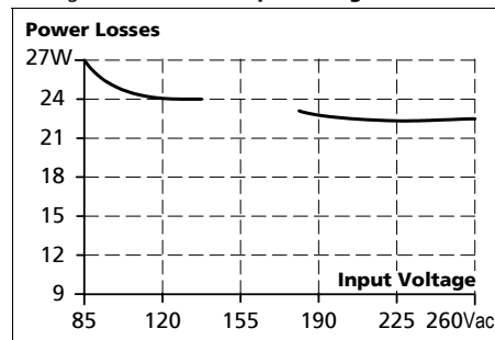
Fig. 9-4 Losses vs. input voltage, 48V, 5A
