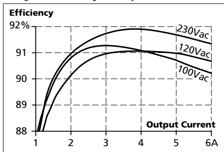
Fig. 9-1 Efficiency vs. output current at 48V
