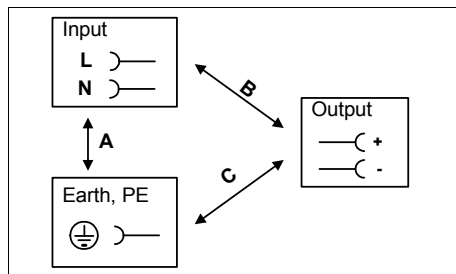
Fig. 18-1 Dielectric strength
