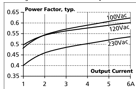
Fig. 5-4 Power Factor vs. output load
