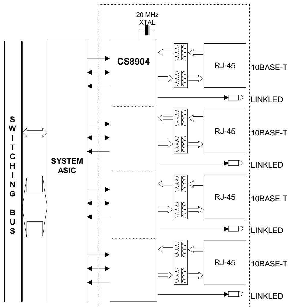
Figure 1. Ethernet Switching Hub Application of CS8904
