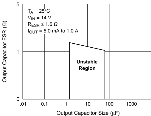
Figure 22. Regulator 1 Stability
