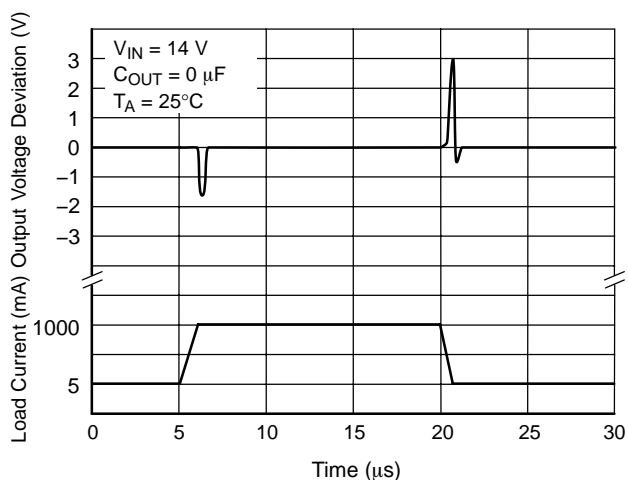
Figure 18. Regulator 1 Load Transient Response
