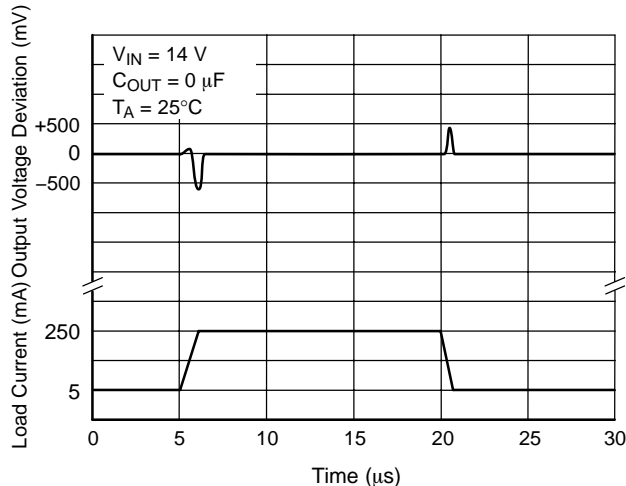
Figure 19. Regulator 2 Load Transient Response
