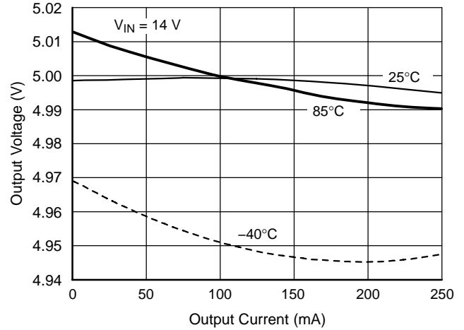
Figure 13. Regulator 2 Load Regulation
