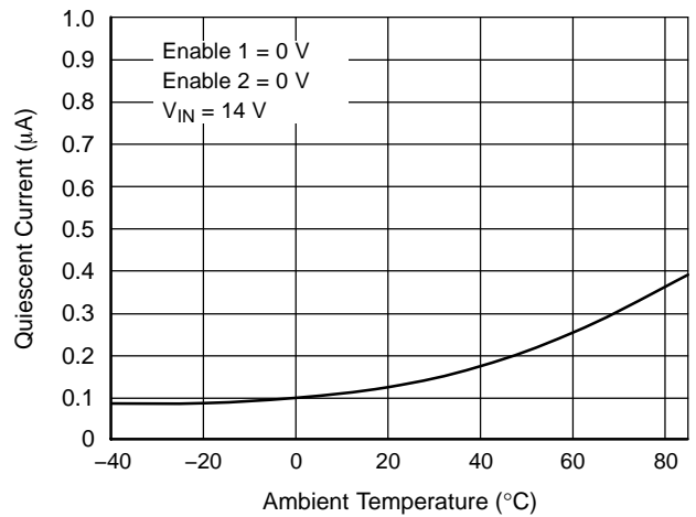
Figure 9. Quiescent Current
