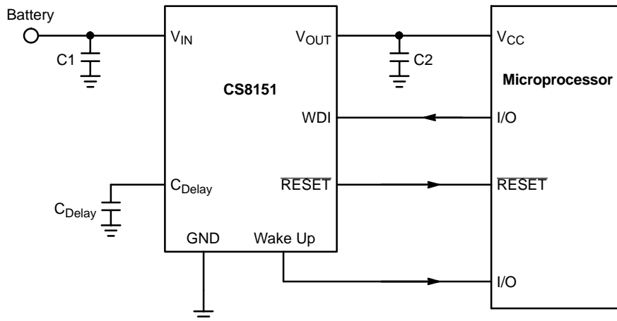
Figure 10. Application Diagram
