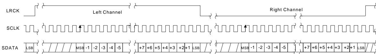
Figure 19. CS4341 Formats 3-6 - Right Justified
