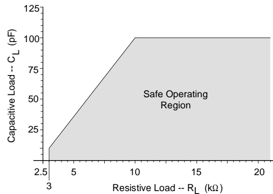
Figure 2. Maximum Loading
