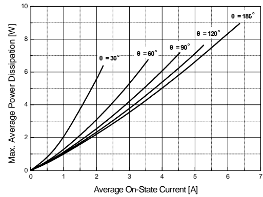
Fig 8. Power Dissipation
