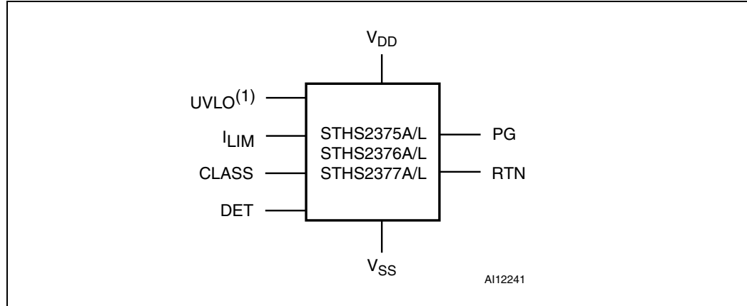
Figure 1. Logic diagram
