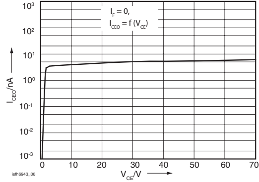
Figure 6. Collector-Emitter Leakage Current (typ.)
