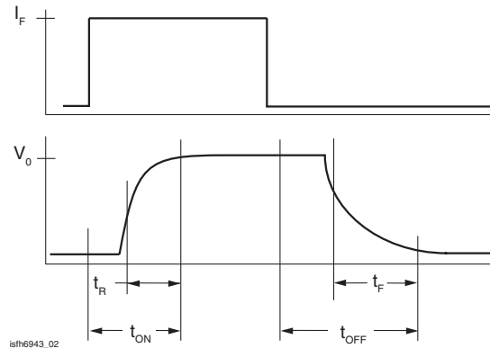
Figure 2. Switching Waveform
