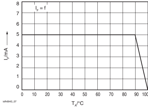
Figure 7. Permissible Forward Current Diode
