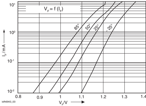
Figure 3. LED Current vs. LED Voltage
