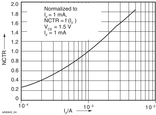
Figure 4. Non-Saturated Current Transfer
