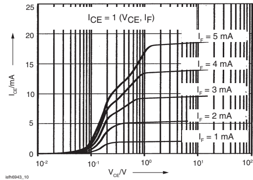
Figure 10. Transistor Output Characteristics
