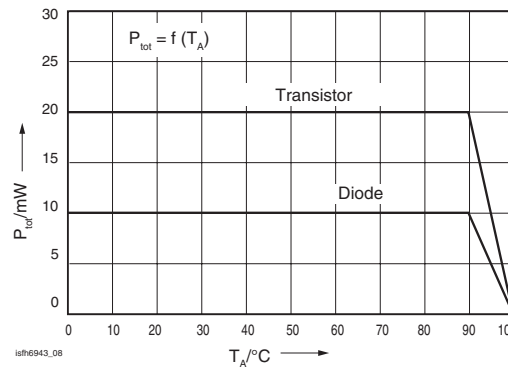
Figure 8. Permissible Power Dissipation
