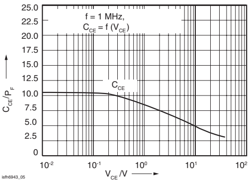
Figure 5. Transistor Capacitances (typ.)
