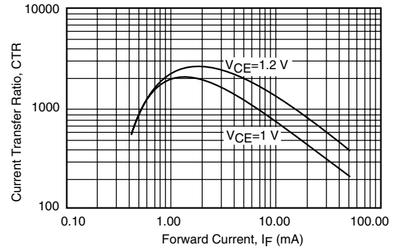
Fig. 7 - Current Transfer Ratio vs. Forward Current
