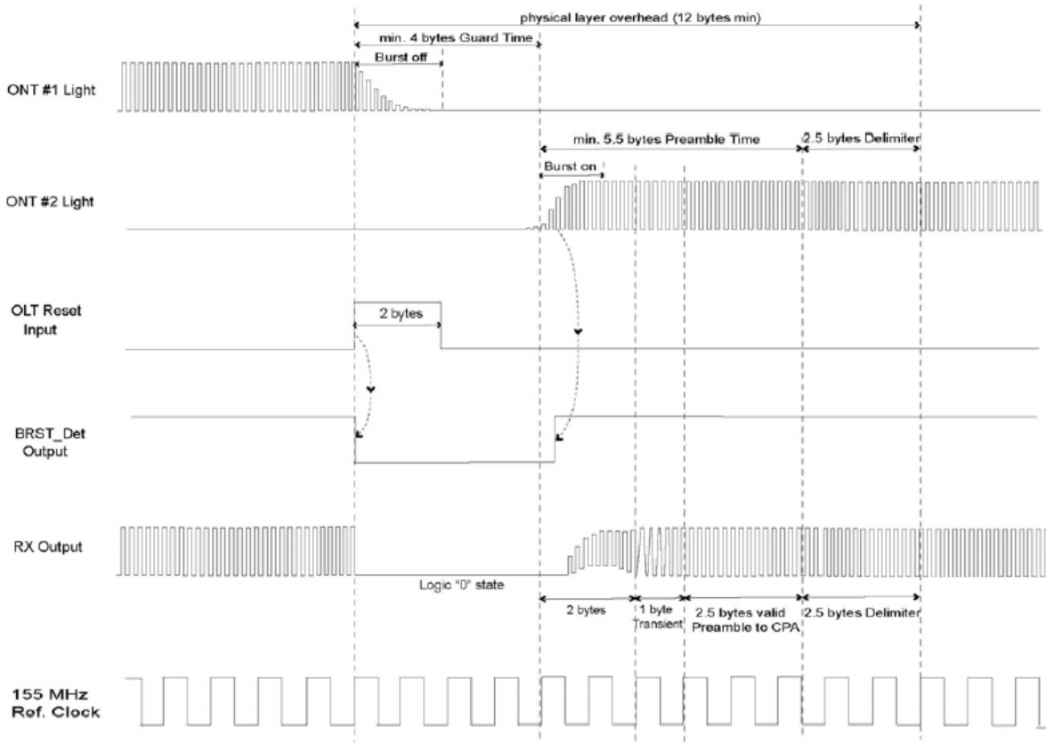
Figure 1. Timing Diagram
