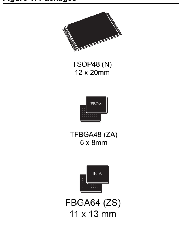
Figure 1. Packages
