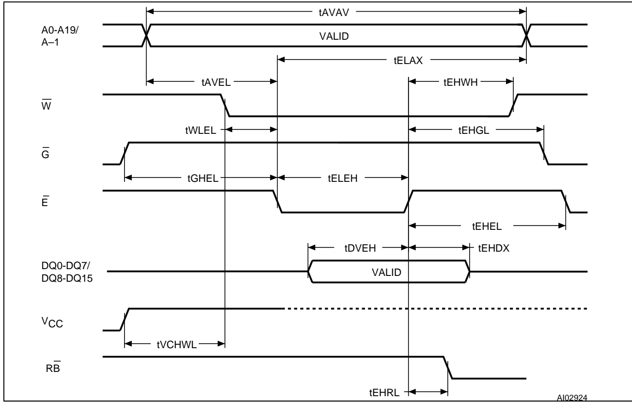
Figure 14. Write AC Waveforms, Chip Enable Controlled
