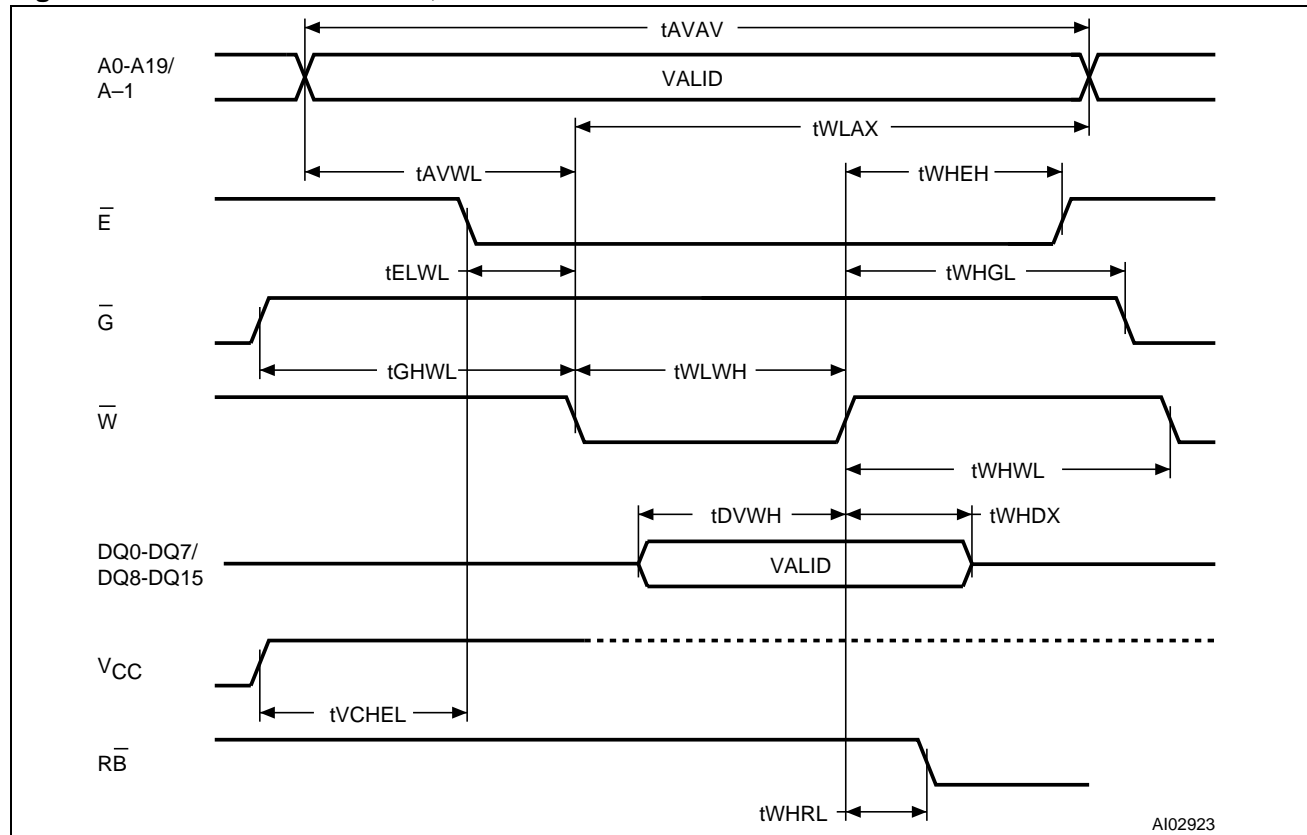
Figure 13. Write AC Waveforms, Write Enable Controlled
