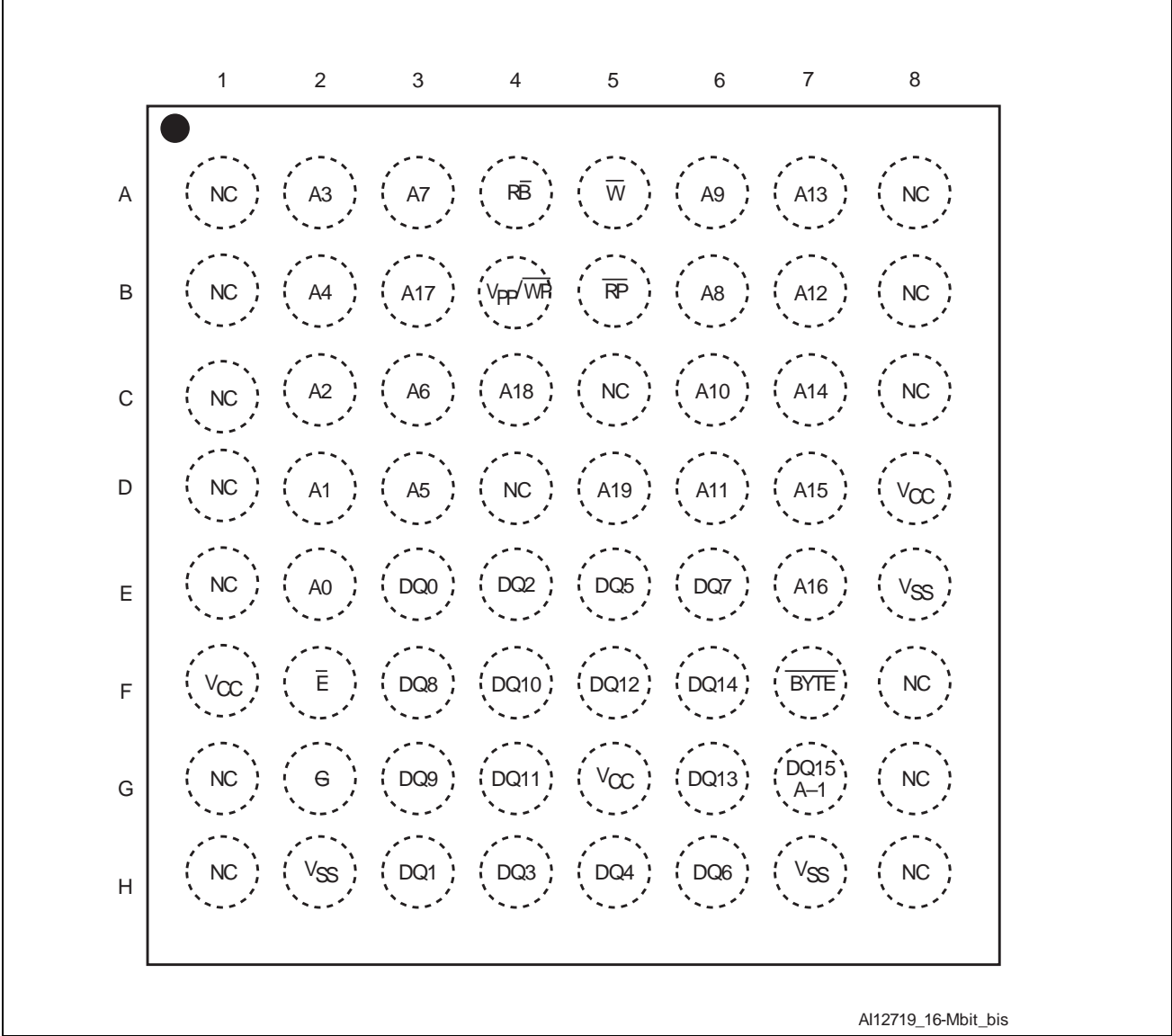
Figure 5. FBGA 64-ball Connections (Top view through package)
