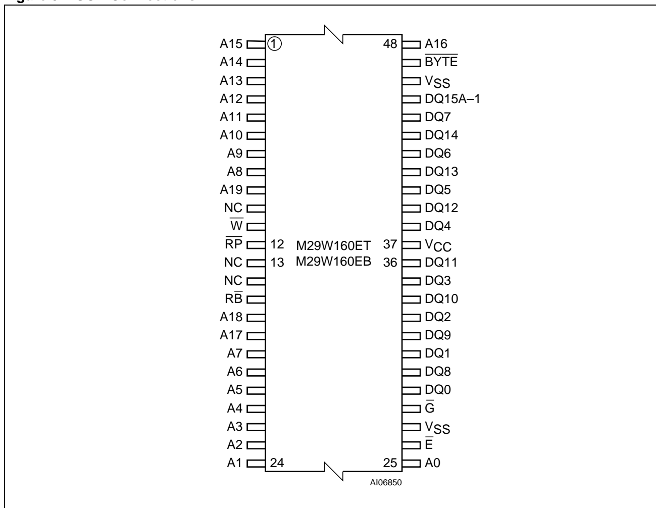
Figure 3. TSOP Connections
