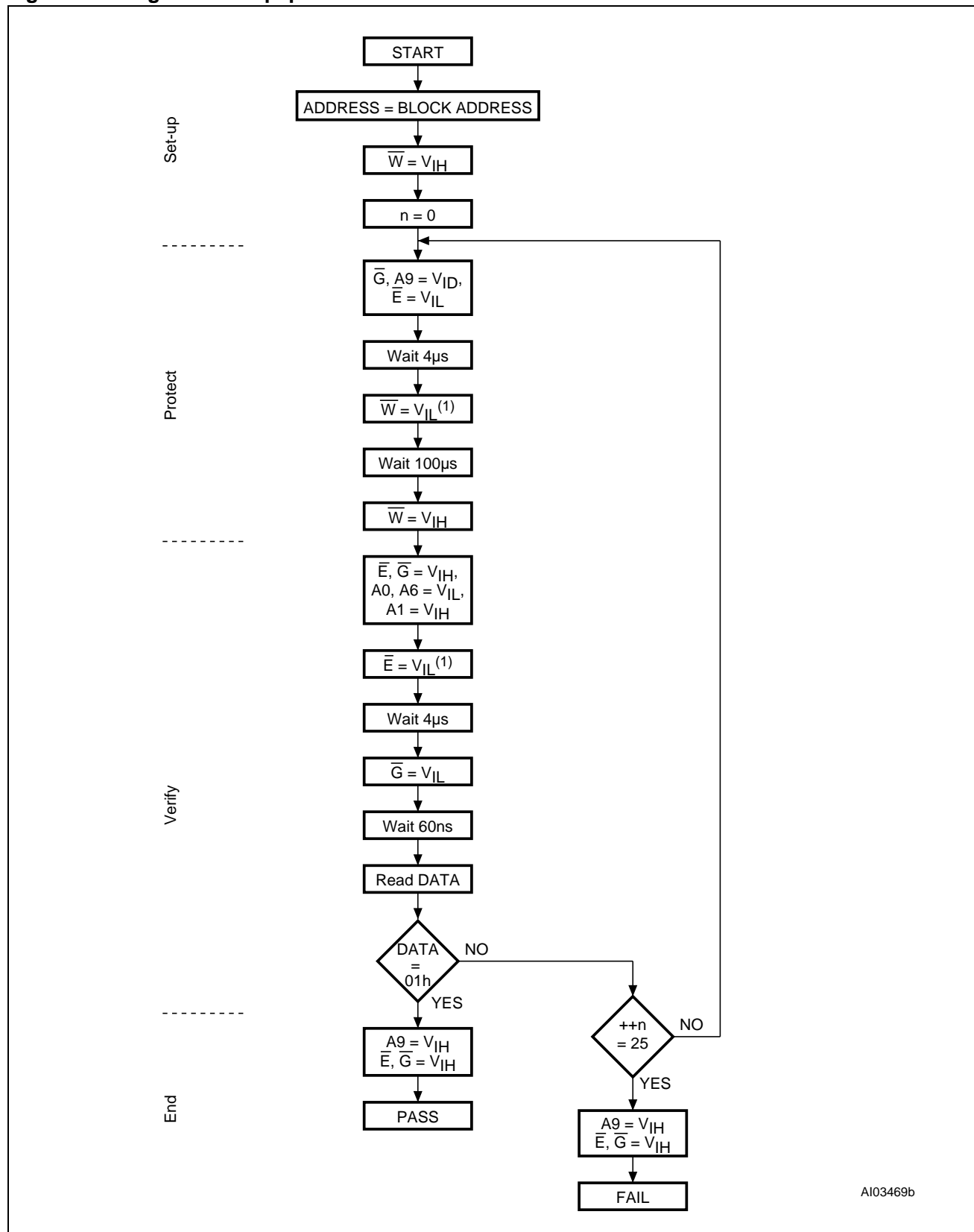
Figure 19. Programmer Equipment Block Protect Flowchart
