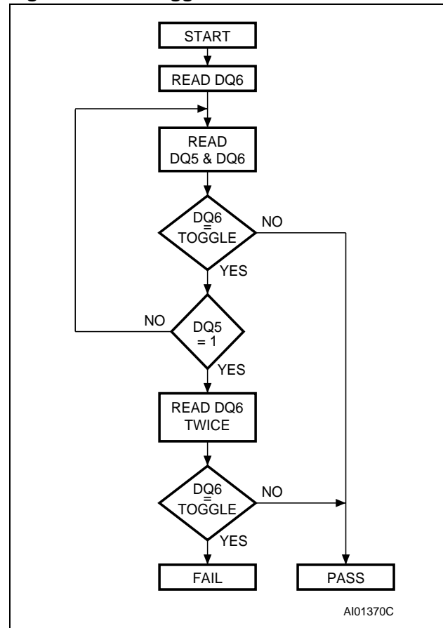
Figure 9. Data Toggle Flowchart
