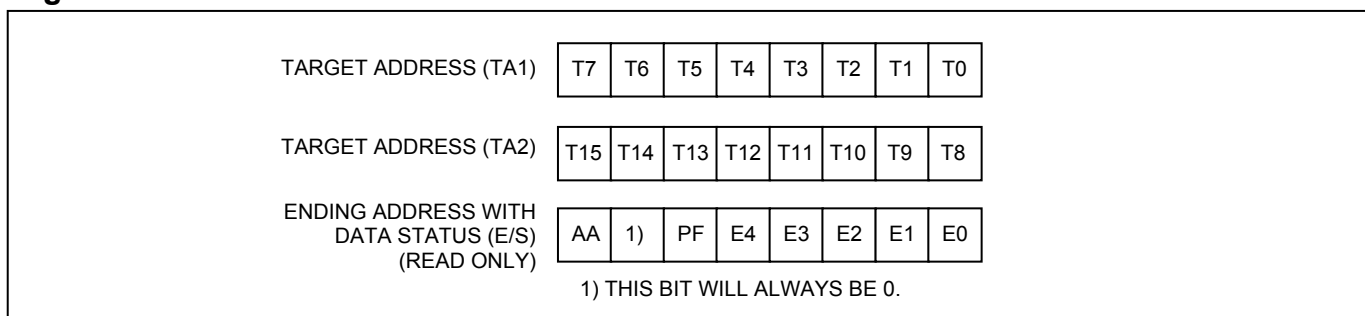
Figure 6. ADDRESS REGISTER
