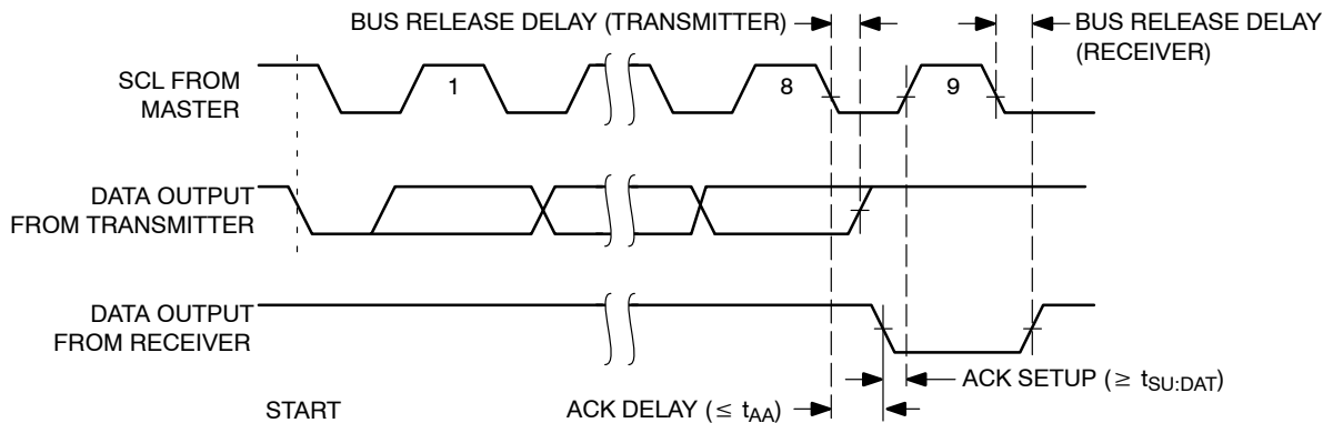
Figure 4. Acknowledge Timing
