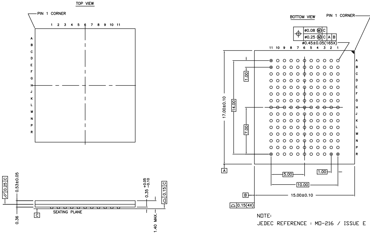
Figure 9. 165-Ball FBGA (15 x 17 x 1.4 mm)
