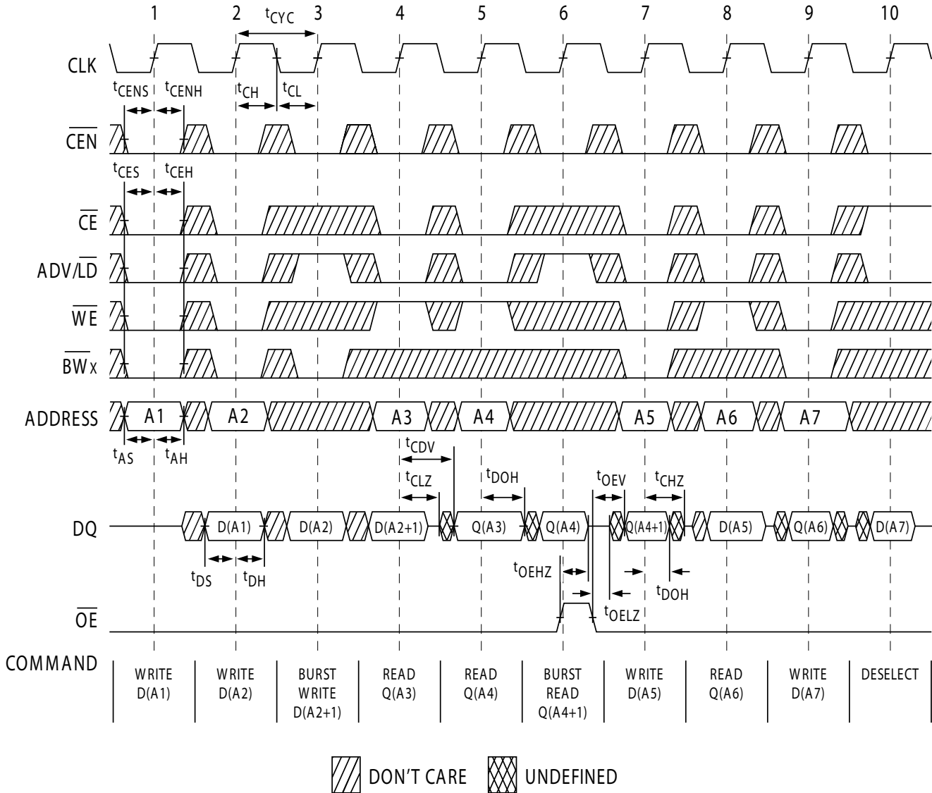
Figure 5. Read/Write Timing
