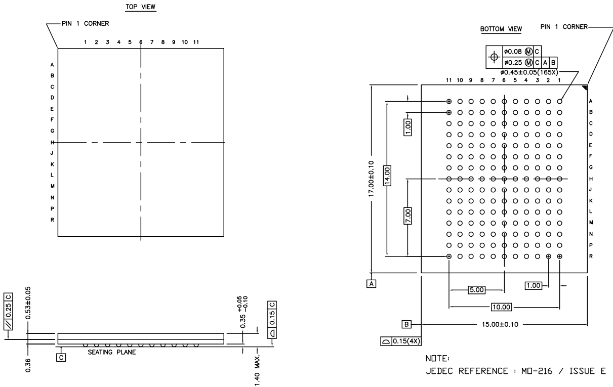
Figure 2. 165-Ball FBGA (15 x 17 x 1.4 mm), 51-85165
