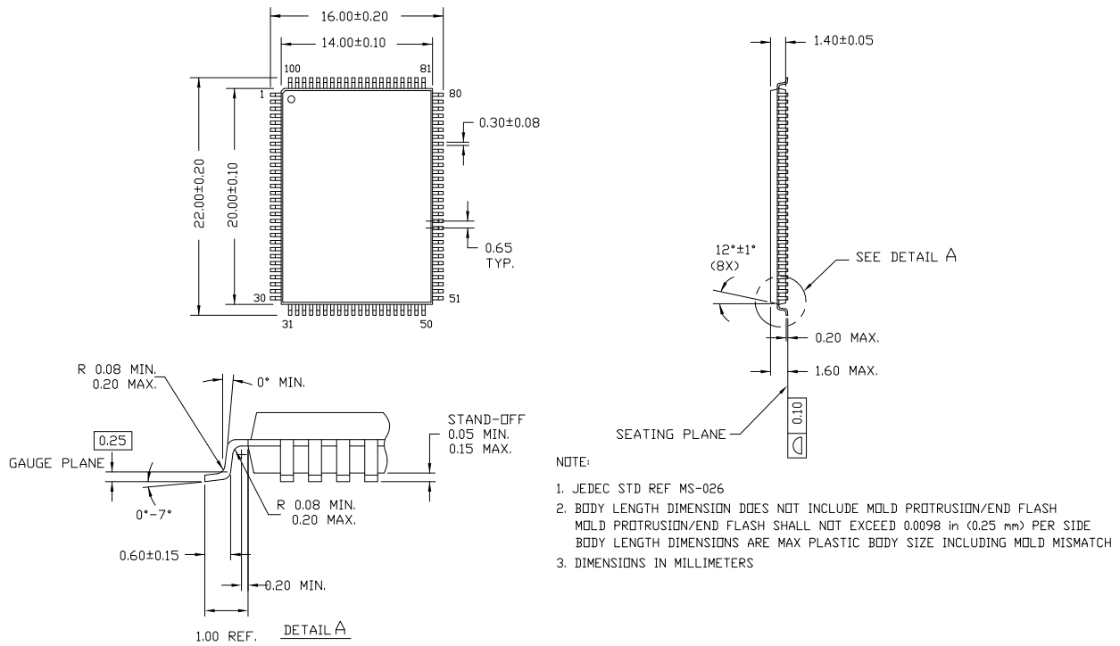
Figure 1. 100-Pin Thin Plastic Quad Flatpack (14 x 20 x 1.4 mm), 51-85050
