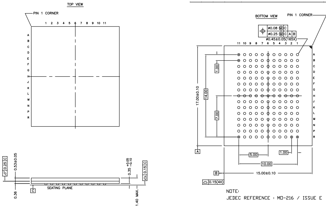
Figure 9. 165-Ball FBGA (15 x 17 x 1.4 mm)
