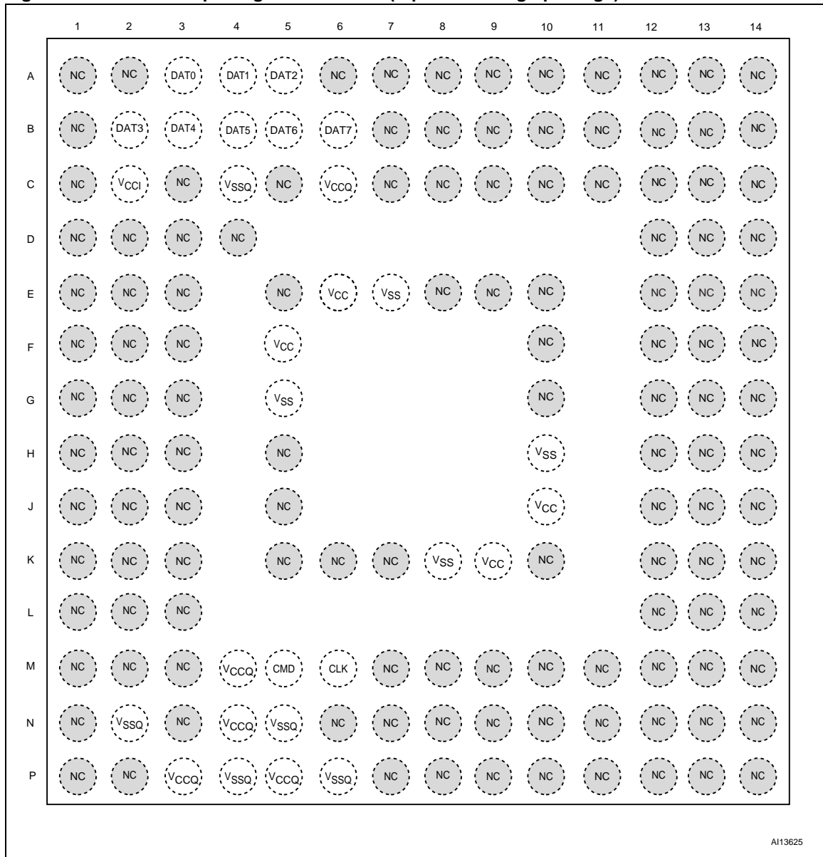
Figure 2. LFBGA153 package connections (top view through package)
