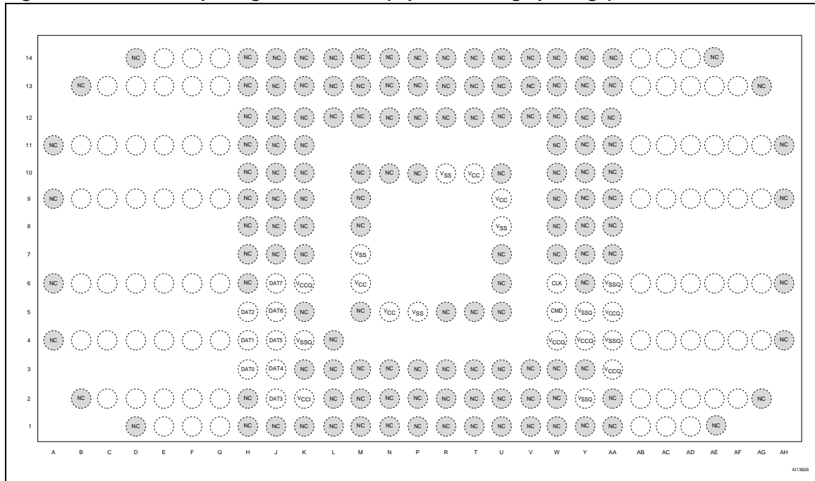
Figure 3. LFBGA169 package connections (top view through package)
