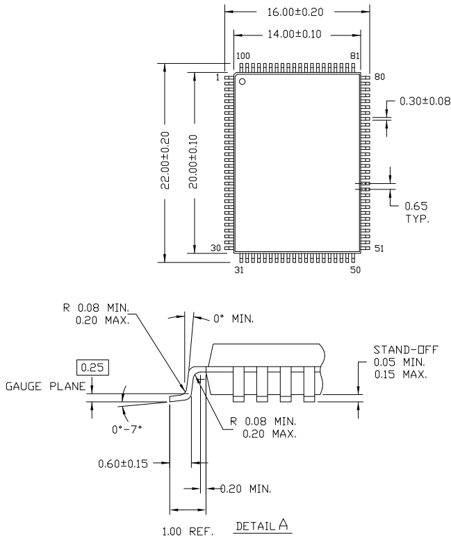
Figure 8. 100-pin TQFP (14 × 20 × 1.4 mm), 51-85050
