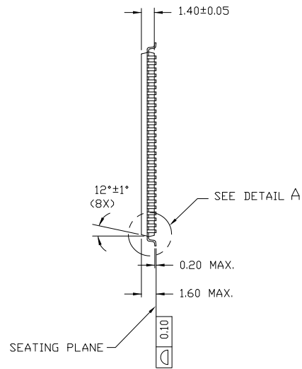
Figure 8. 100-pin TQFP (14 × 20 × 1.4 mm), 51-85050
