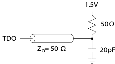
Figure 7. 3.3V TAP AC Output Load Equivalent
