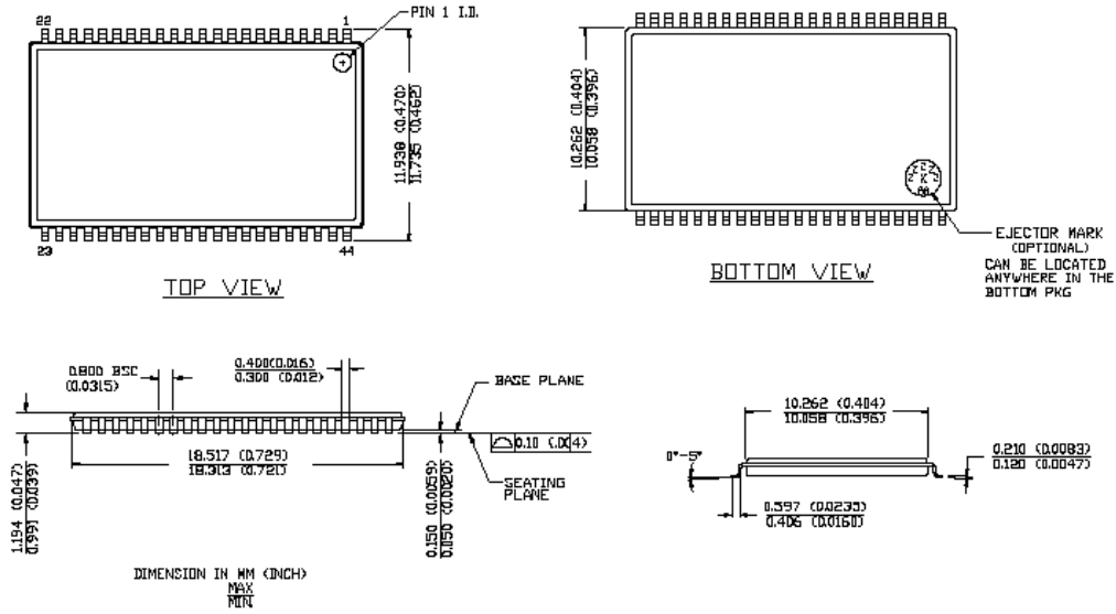
Figure 14. 44-Pin TSOP II (51-85087)
