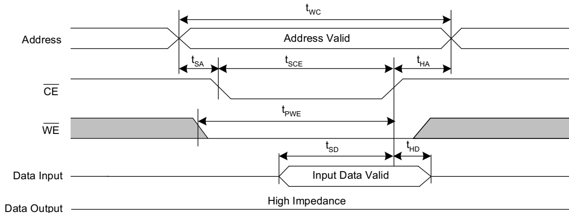
Figure 8. SRAM Write Cycle #2: \overline{CE} Controlled [18, 19, 20]
