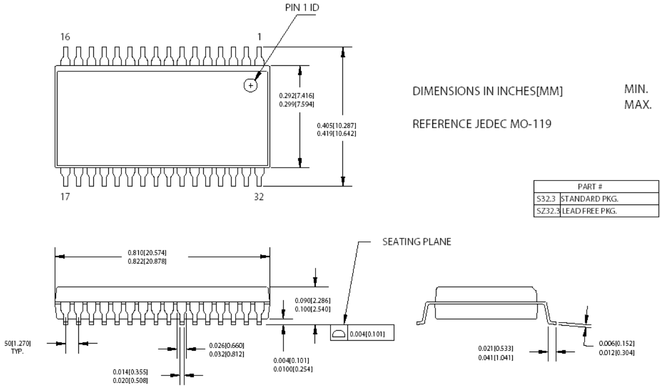
Figure 16. 32-Pin SOIC (51-85127)
