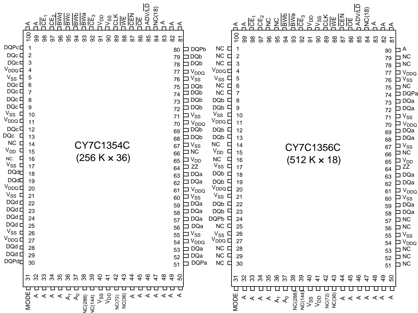
Figure 1. 100-pin TQFP
