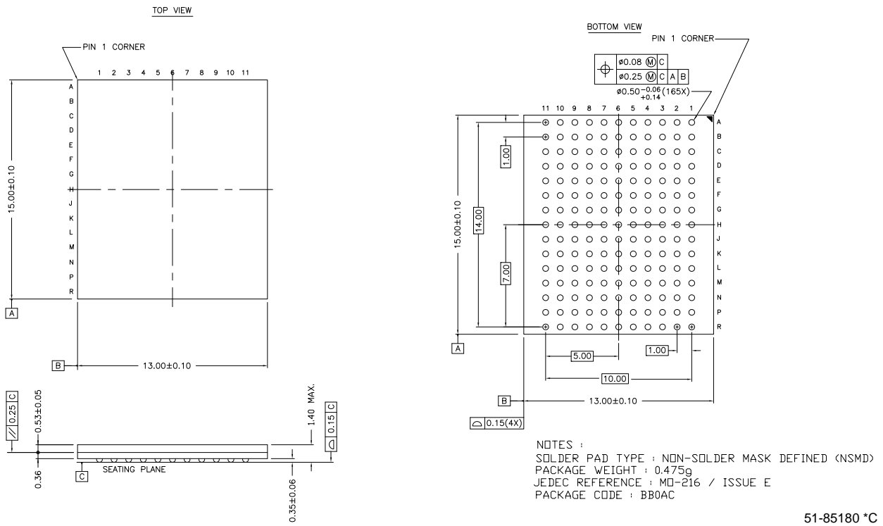
Figure 10. 165-ball FBGA (13 x 15 x 1.4 mm), 51-85180
