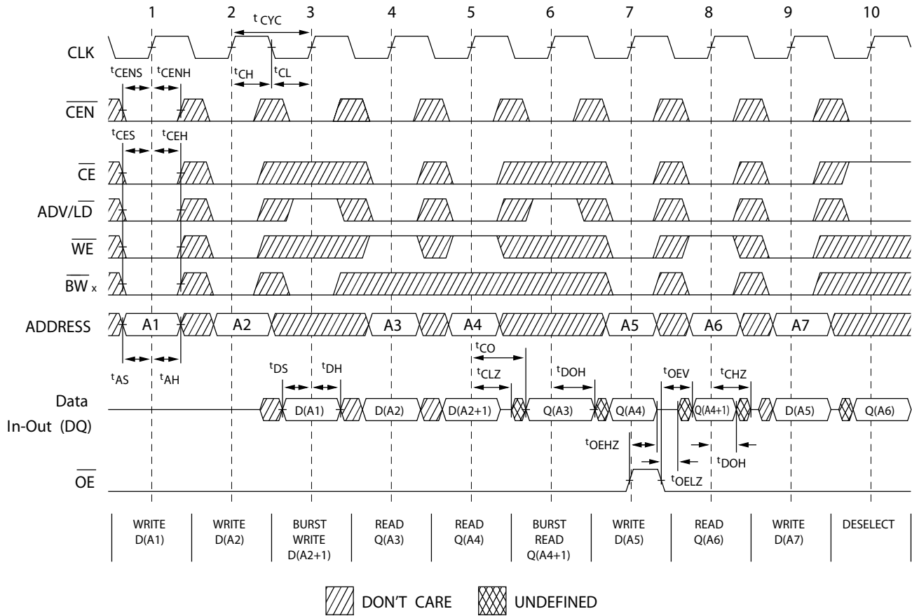
Figure 5. Read/Write Timing [28, 29, 30]
