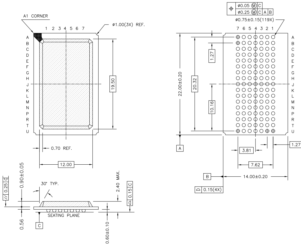
Figure 9. 119-ball BGA (14 x 22 x 2.4 mm), 51-85115
