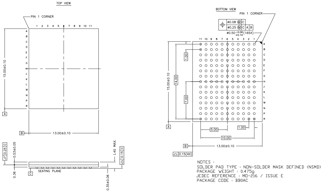
Figure 3. 165-ball FBGA (13 x 15 x 1.4 mm), 51-85180
