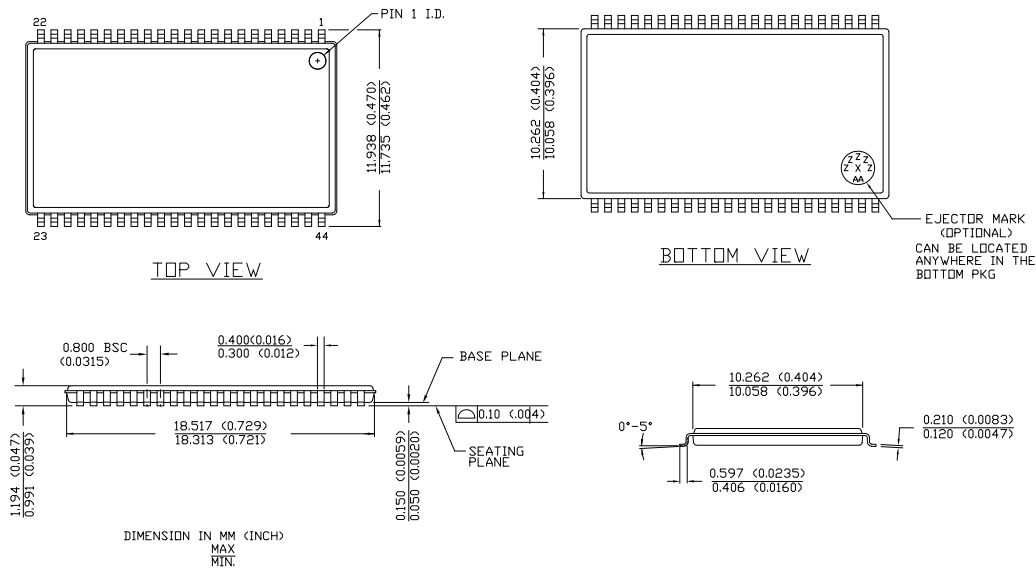
Figure 2. 44-pin TSOP II (51-85087)
