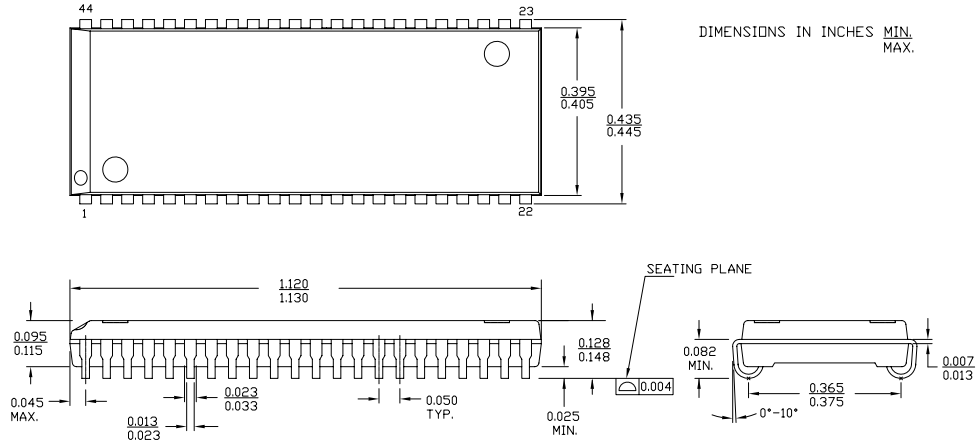
Figure 2. 44-pin TSOP II (51-85087)
