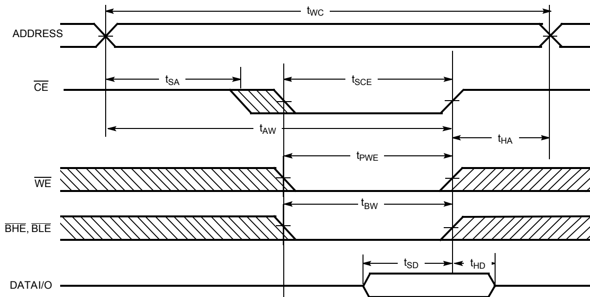
Figure 6. Write Cycle No. 1 ( \overline{\text{CE}} Controlled) [24, 25]
