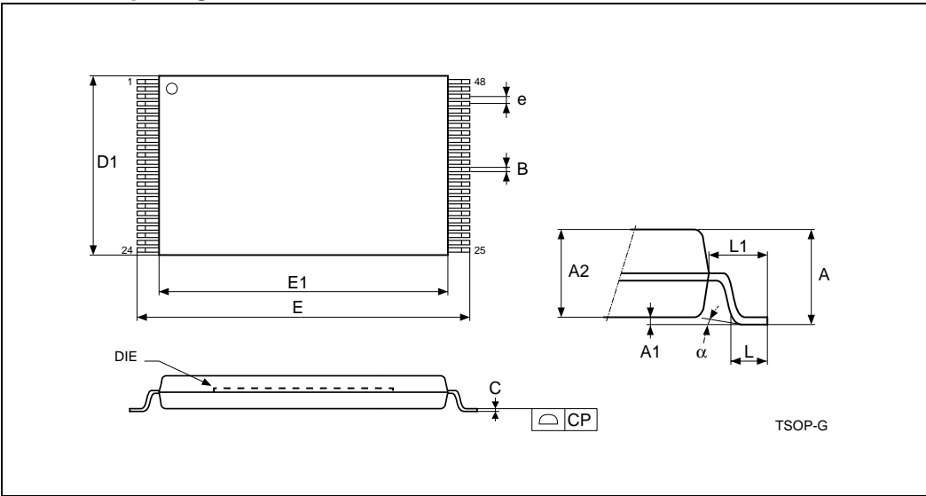
Figure 14. TSOP48 – 48 lead Plastic Thin Small Outline, 12 x 20mm, top view package outline
