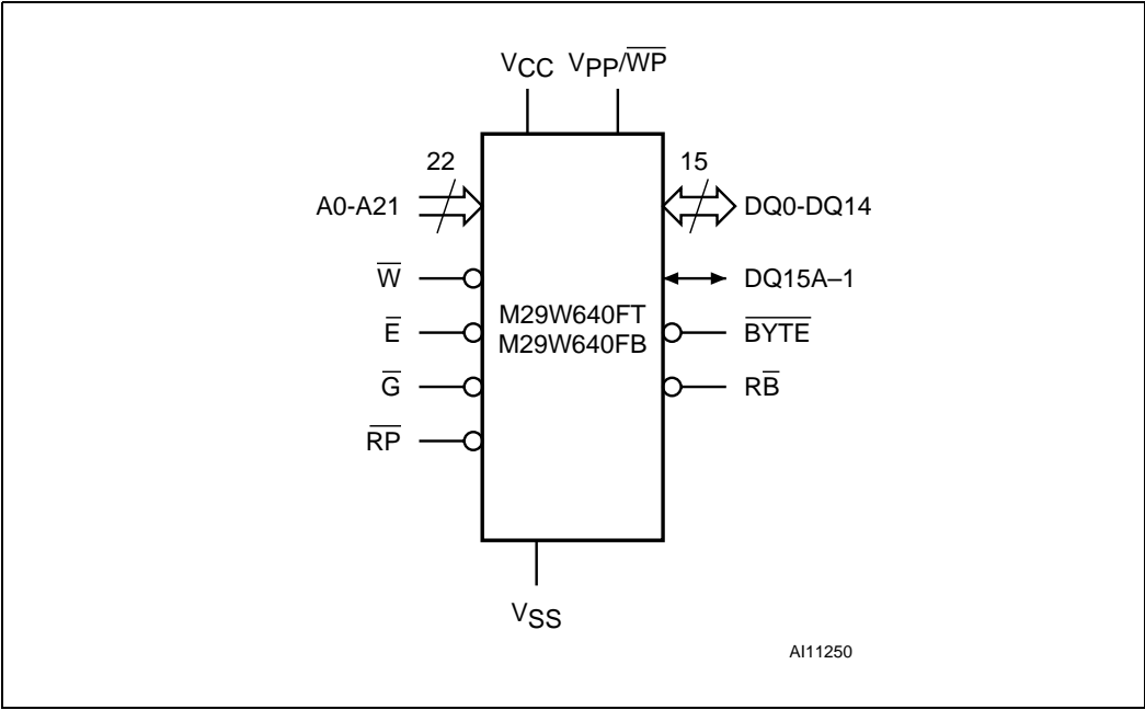
Figure 1. Logic diagram
