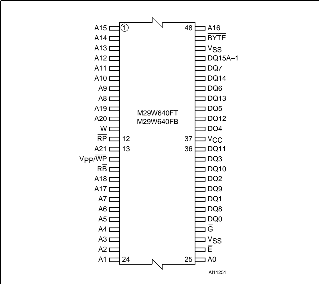
Figure 2. TSOP connections
