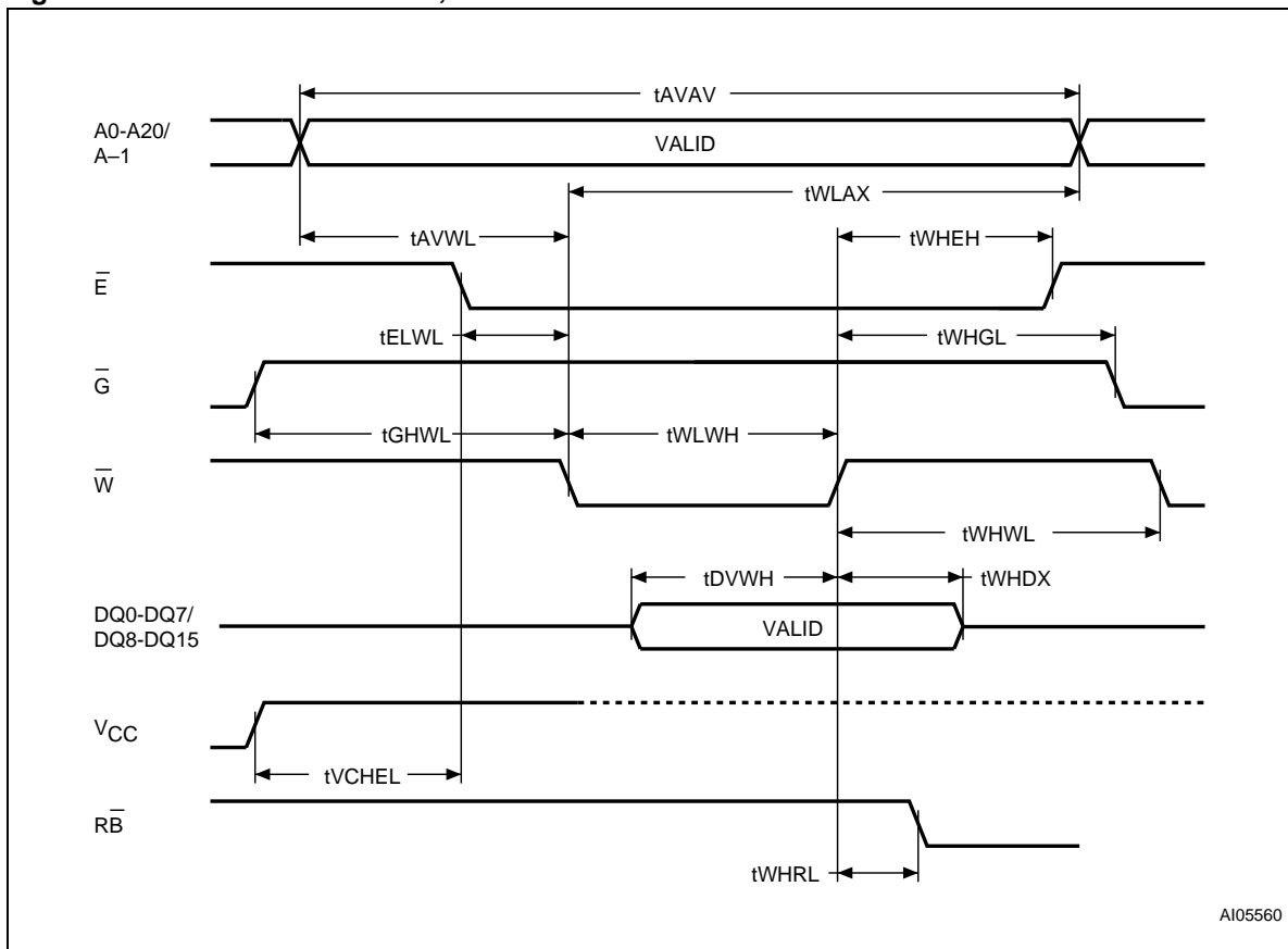
Figure 10. Write AC waveforms, Write Enable controlled
