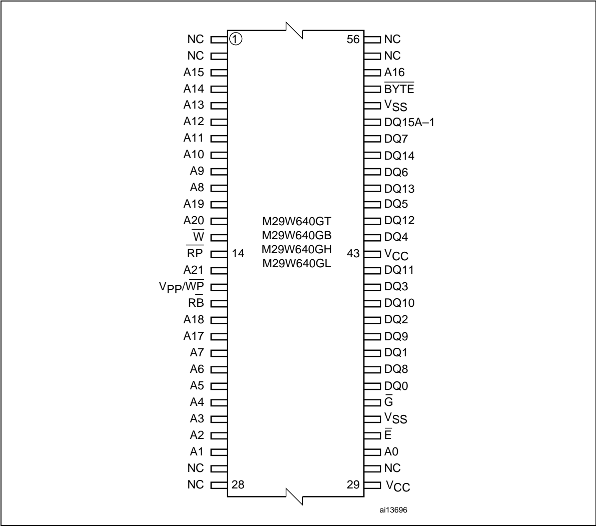
Figure 3. TSOP56 connections
