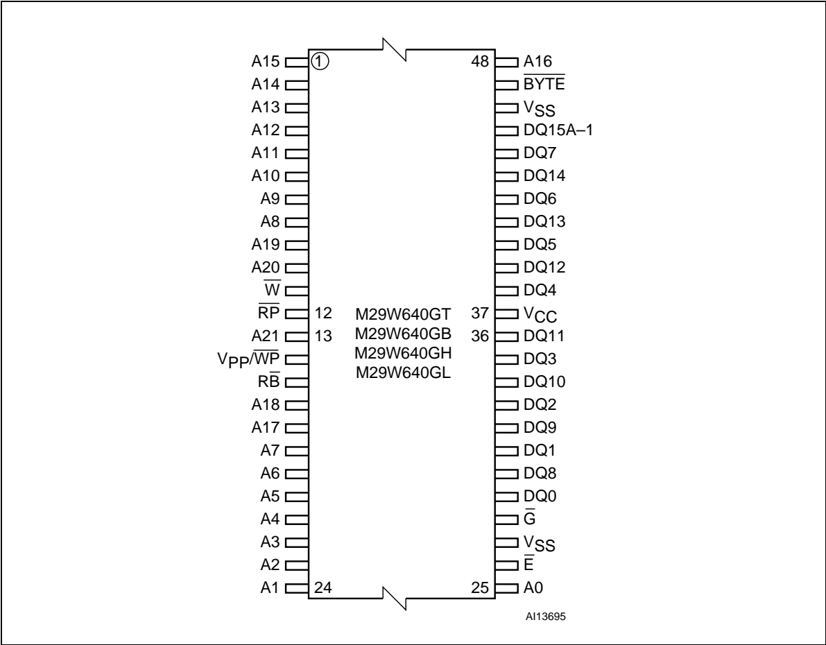
Figure 2. TSOP48 connections
