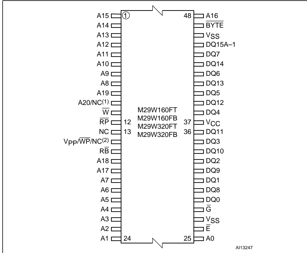
Figure 2. TSOP connections
