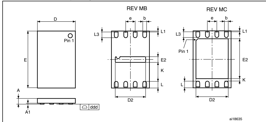
Figure 25. UFDFPN8 (MLP8) – 8-lead ultra thin fine pitch dual flat package no lead 2 × 3mm, package outline
