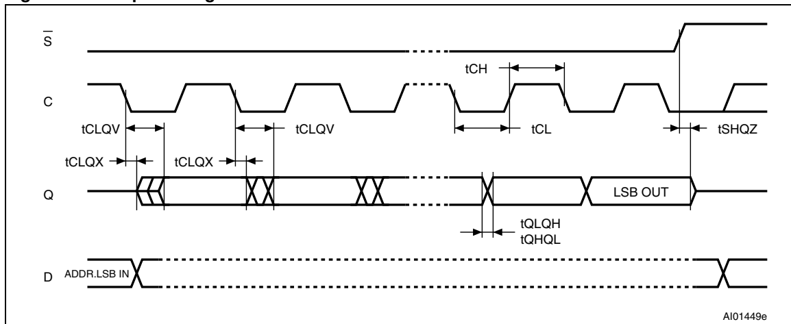
Figure 22. Output timing
