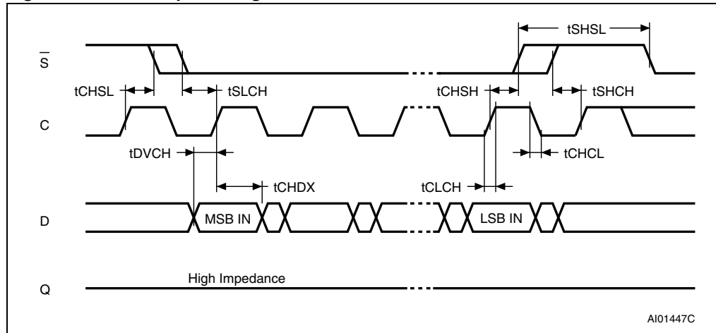
Figure 21. Hold timing
