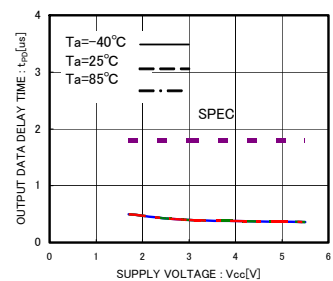
Fig.23 'H' Data output delay time t p01
