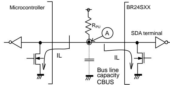
Fig.49 I/O circuit diagram
