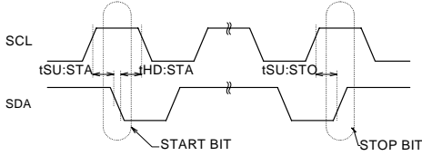
Fig.1-(b) Start-stop bit timing
