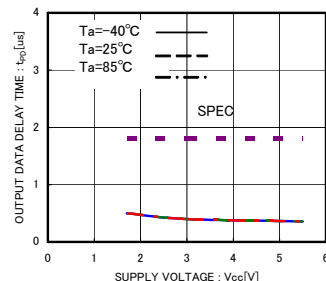
Fig.22 'L' Data output delay time t p0
