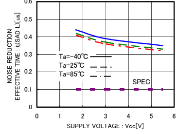
Fig.29 Noise reduction effective time t_1(SDA L)
