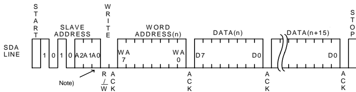
Fig.35 Page write cycle (BR24S16-W)
