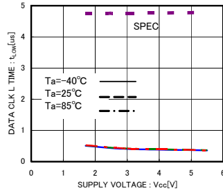
Fig.15 Data clock Low Period t LOW
