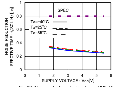
Fig.26 Noise reduction effective time t_1(SCL H)
