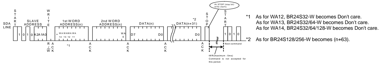
Fig.39 Page write cycle(BR24S32/64/128/256-W)
