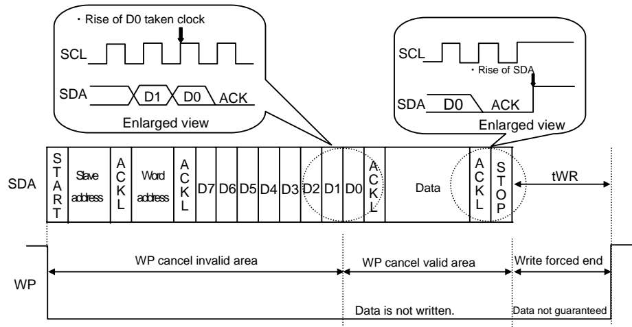
Fig.47 WP valid timing
