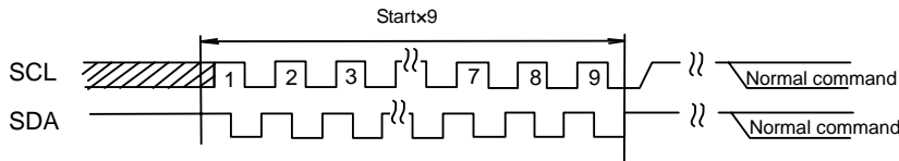
Fig.48-(c) STARTx9+ command input
