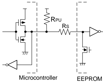
Fig.53 I/O circuit diagram
