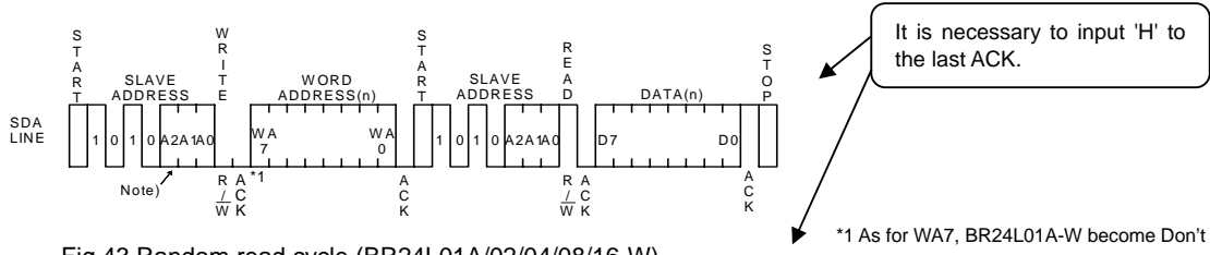
Fig.43 Random read cycle (BR24L01A/02/04/08/16-W)
