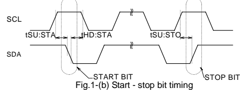
Fig.1-(b) Start - stop bit timing
