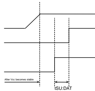
Fig.58 When SCL='H' and SDA='L'
