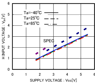
Fig.3 'H' input voltage V_{IH} (A0,A1,A2,SCL,SDA,WP)
