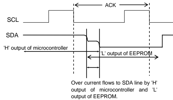
Fig.54 Input / output collision timing
