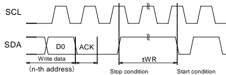
Fig.1-(c) Write cycle timing
