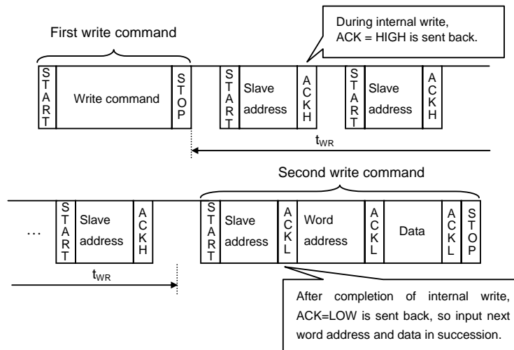
Fig.49 Case to continuously write by acknowledge polling
