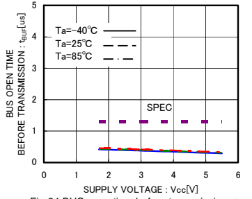
Fig.24 BUS open time before transmission t_{BUF}
