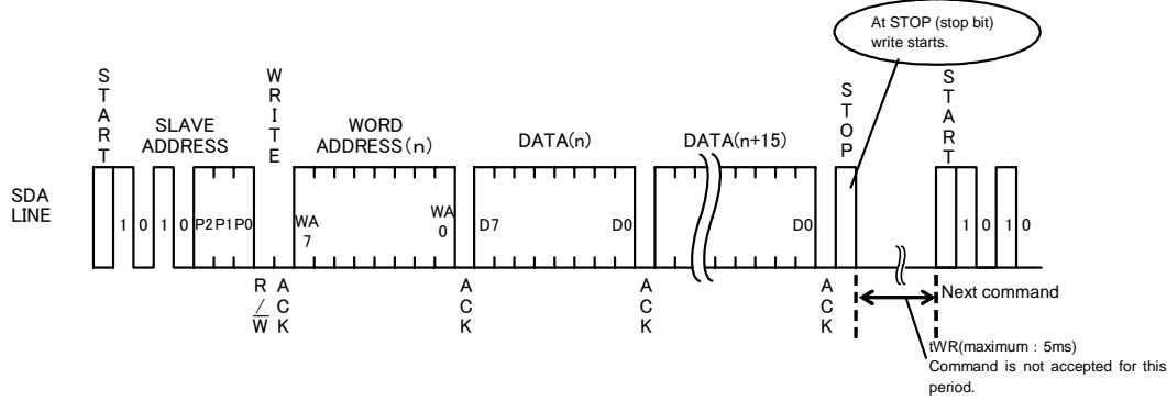
Fig.38 Page write cycle(BR24S16-W)
