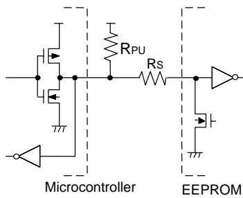
Fig.50 I/O circuit diagram
