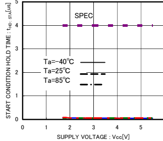
Fig.16 Start Condition Hold Time t HD:STA
