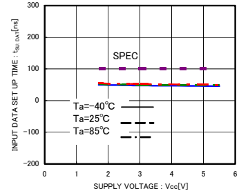
Fig.20 Input Data Setup Time t SU:DAT (HIGH)
