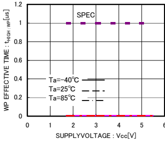
Fig.31 WP effective time t_{HIGH:WP}
