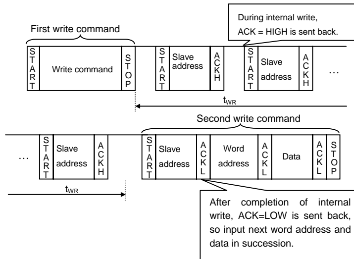
Fig.46 Case to continuously write by acknowledge polling
