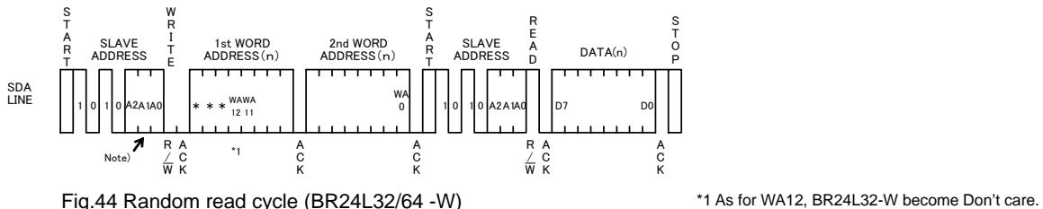
Fig.44 Random read cycle (BR24L32/64 -W)
