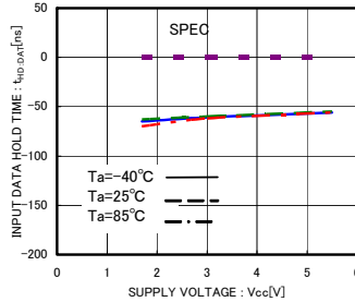
Fig.19 Input Data Hold Time t HD:DAT (LOW)
