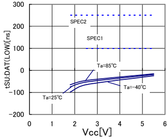
Fig.24 Input data setup time tSU:DAT(LOW)
