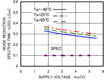
Fig.27 Noise reduction effective time t_1(SCL L)
