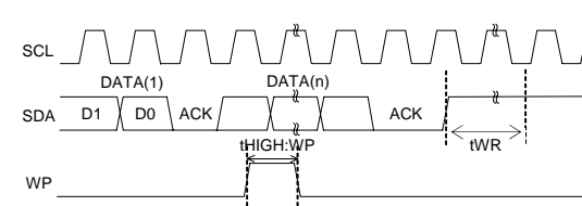
Fig.1-(d) WP timing at write execution
