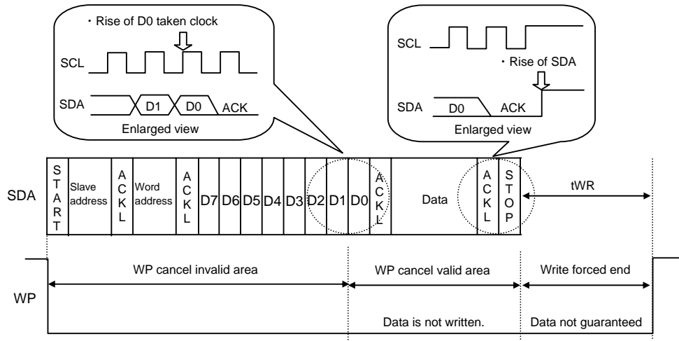
Fig.50 WP valid timing
