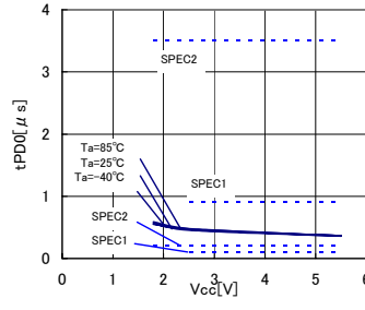
Fig.25 Output data delay time tPDO
