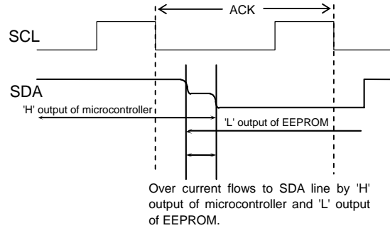
Fig.51 Input/output collision timing
