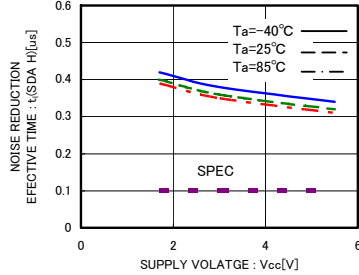
Fig.28 Noise reduction effective time t_1(SDA H)
