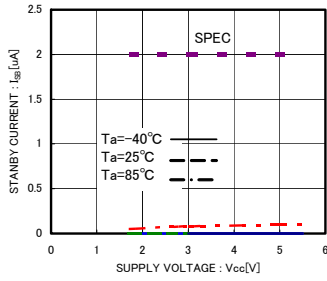
Fig.12 Standby operation I SB
