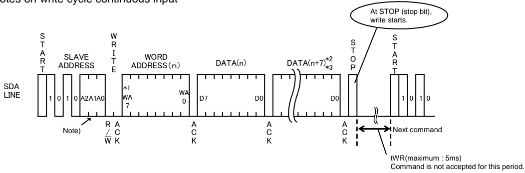
Fig.41 Page write cycle
