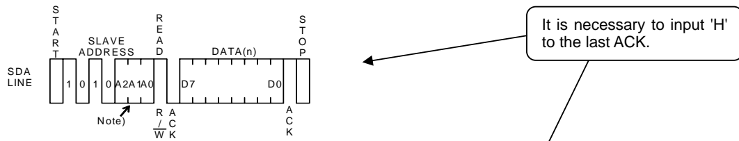
Fig.42 Current read cycle
