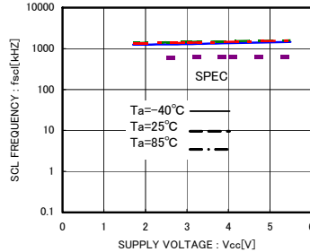
Fig.13 SCL frequency f SCL
