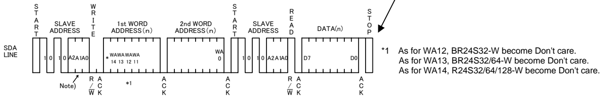
Fig.41 Random read cycle (BR24S32/64/128/256-W)
