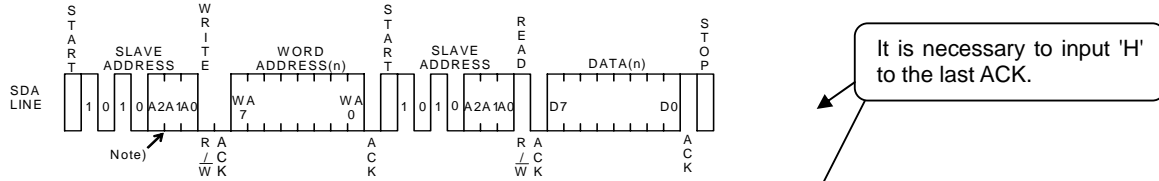
Fig.40 Random read cycle (BR24S16-W)
