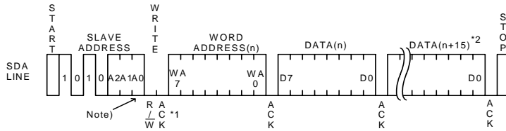
Fig.38 Page write cycle (BR24L01A/02/04/08/16-W)
