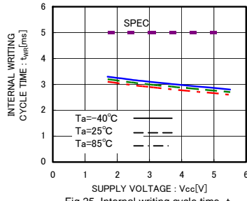
Fig.25 Internal writing cycle time t_{WR}
