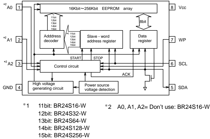
Fig.2 Block diagram
