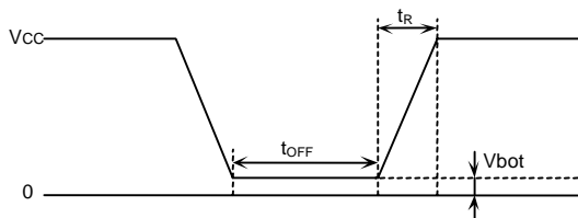
Fig.60 Rise waveform diagram
