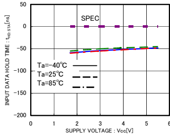
Fig.18 Input Data Hold Time t HD:DAT (HIGH)
