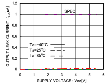
Fig.8 Output leak current I_{OI} (SDA)
