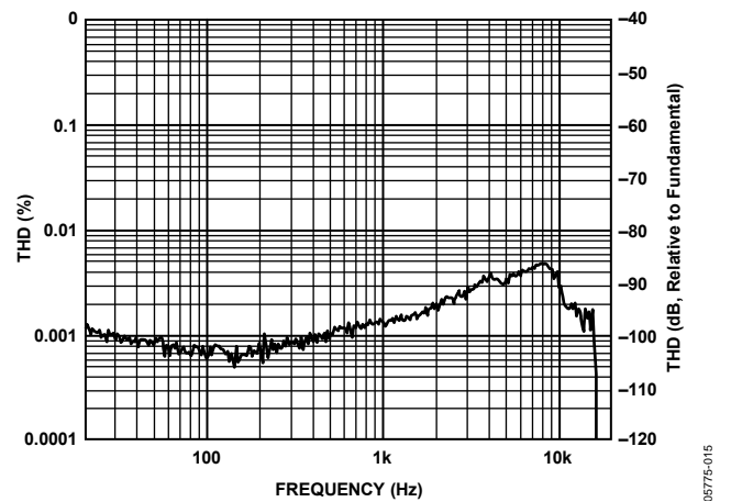
Figure 15. THD vs. Frequency, 1 W Output Power into 8 Ω Load, PVDD = 12 V
