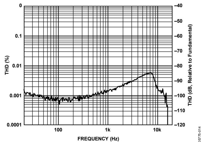
Figure 14. THD vs. Frequency, 1 W Output Power into 6 Ω Load, PVDD = 12 V
