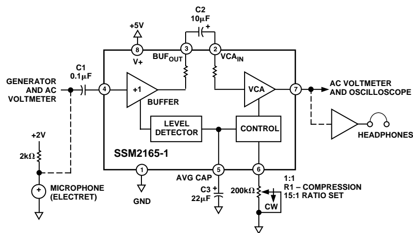
Figure 8. Electret Microphone Preamp Example
