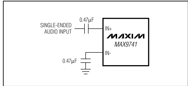
Figure 4. Single-Ended Input
